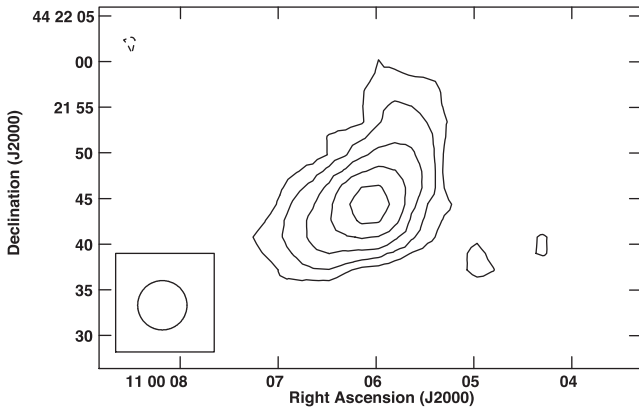
Figure 4. 1.4-GHz VLA map of J1100+4421 from the FIRST survey (Becker et al. 1995). The observation was performed on 1997 February 25. The peak brightness is 8.3 \text{ mJy beam}^{-1} , the restoring beam is circular with FWHM size of 5.4 arcsec, and shown in the lower left-hand corner of the image. The lowest contour levels are at \pm 0.4 \text{ mJy beam}^{-1} at 3\sigma image noise level, further positive contour levels increase by a factor of 2. The dashed line represents negative contour.
