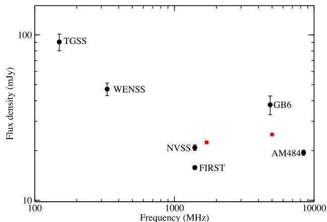
Figure 5. Non-contemporaneous radio flux density measurements of J1100+4421. Black circles show data from various surveys such as the Giant Meterwave Radio Telescope 150 MHz all-sky radio survey (TGSS, Intema et al. 2017), the Westerbork Northern Sky Survey (WENSS, Rengelink et al. 1997), the NVSS, the FIRST and the Green Bank 4.85 GHz survey (GB6, Gregory et al. 1996), and the flux density from the archival 8.4-GHz VLA observation (project code: AM484). Red squares (grey squares in the printed version) show the sum of the flux density of the fitted components of our EVN data.
