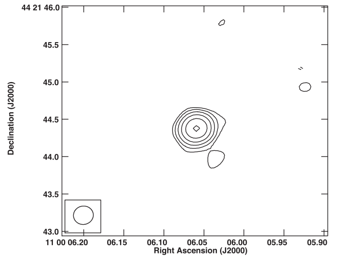
Figure 3. 8.4-GHz VLA image of J1100+4421. The observation was performed on 1995 August 15. The peak brightness is 18.4 \text{ mJy beam}^{-1} . The FWHM size of the restoring beam is 0.27 \times 0.25 \text{ arcsec}^2 at a position angle of -81^\circ , as shown in the bottom left-hand corner of the image. The lowest contours are at \pm 0.5 \text{ mJy beam}^{-1} corresponding to 3\sigma image noise level, further positive contour levels increase by a factor of 2.
