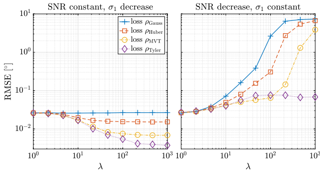
Fig. 3. For \epsilon -contaminated array data \epsilon = 0.05 with one source, RMSE vs. outlier strength \lambda for each loss function for (left): ASNR= 25 dB and background noise \sigma_1 is decreasing, and (right): Background noise \sigma_1 is fixed and outlier noise \lambda\sigma_1 is increasing (at \lambda = 1 : ASNR= 25 dB; and at \lambda = 10^3 : ASNR = 25 - 10 \log(1 - \epsilon + \epsilon\lambda^2) = -22 dB). RMSE evaluation based on N_{\text{run}} = 250 simulation runs.
