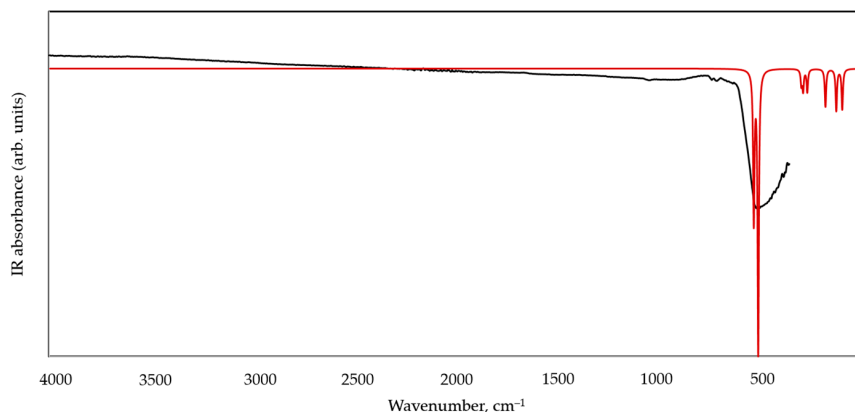
Figure 10. IR spectra of \text{BaOsF}_6 : experimentally observed (black) and calculated with DFT-PBE0 (red).
