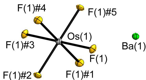
Figure 8. Formula unit of \text{BaOsF}_6 . Displacement ellipsoids are shown at 70% probability at 100 K.
