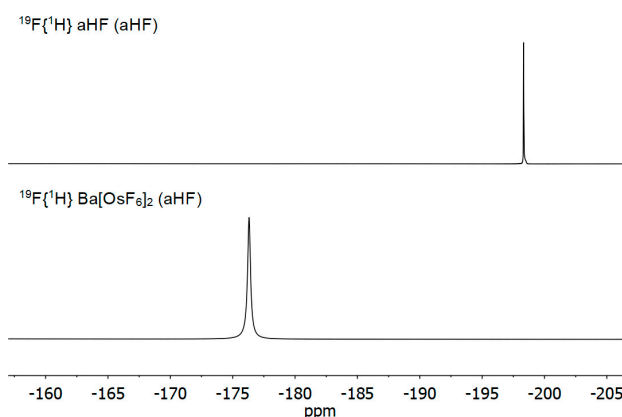
Figure 5. ^{19}\text{F} NMR spectrum of anhydrous HF (top) and \text{Ba}(\text{OsF}_6)_2 in anhydrous HF (bottom).
