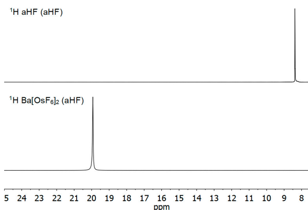
Figure 4. ^1\text{H} NMR spectra of neat anhydrous HF (top) and anhydrous HF with \text{Ba}(\text{OsF}_6)_2 (bottom).
