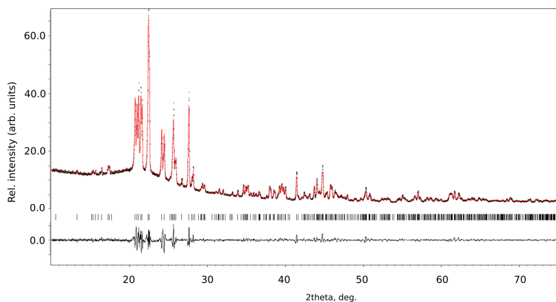
Figure 1. Powder X-ray diffraction pattern (at 293 K) of \text{Ba}(\text{OsF}_6)_2 : the experimental data (black crosses), the Rietveld profile (red), and the differential profile (bottom, black). The calculated reflection positions for \text{Ba}(\text{OsF}_6)_2 are shown as black ticks. R_p = 0.0343 , wR_p = 0.0492 .
