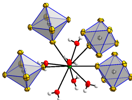
Figure 12. Fragment of the crystal structure of \text{Ba}(\text{OsF}_6)_2 \cdot 6\text{H}_2\text{O} showing the coordination of \text{OsF}_6^- and \text{H}_2\text{O} around \text{Ba}^{2+} . Displacement ellipsoids are shown at 70% probability level at 100 K. All non-hydrogen atoms are shown anisotropic, hydrogen atoms are shown with arbitrary radii.
