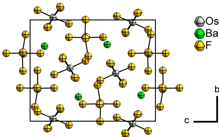
Figure 2. The crystal structure of \text{Ba}(\text{OsF}_6)_2 (projection along a -axis). Atoms are shown with isotropic displacement parameters, F atoms with fixed ones.
