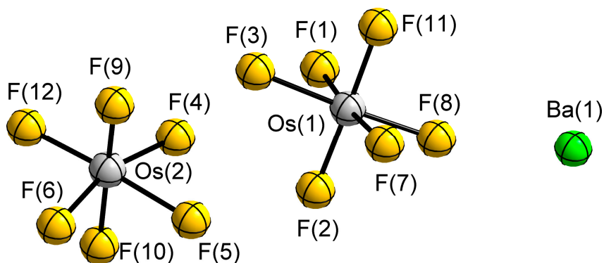
Figure 3. Asymmetric unit of \text{Ba}(\text{OsF}_6)_2 . Atoms are shown with isotropic displacement parameters, F atoms with fixed ones.
