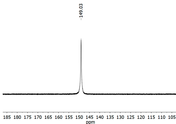
Figure 6. A part of ^{19}\text{F} NMR spectrum of \text{Ba}(\text{OsF}_6)_2 in anhydrous HF showing the \text{OsF}_6^- signal.
