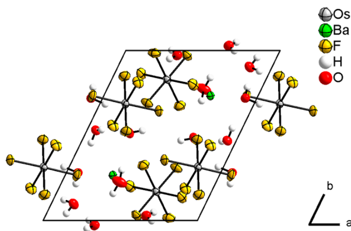
Figure 11. The crystal structure of \text{Ba}(\text{OsF}_6)_2 \cdot 6\text{H}_2\text{O} (projection along c -axis). Displacement ellipsoids are shown at 70% probability level at 100 K. All the non-hydrogen atoms are shown anisotropic, hydrogen atoms are shown with arbitrary radii.
