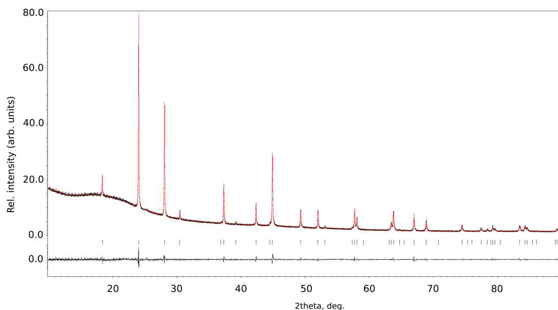
Figure 9. Powder X-ray diffraction pattern (at 293 K) of \text{BaOsF}_6 : the experimental data (black crosses), the Le Bail profile (red), and the differential profile (bottom, black). The calculated reflection positions for \text{BaOsF}_6 are shown as black ticks. R_p = 0.0189 , wR_p = 0.0264 .
