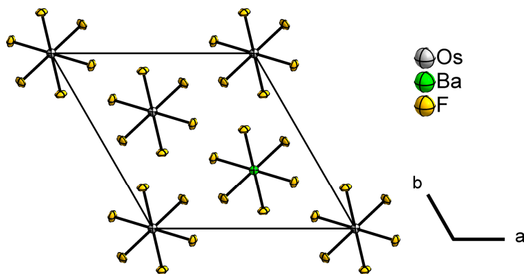
Figure 7. The crystal structure of \text{BaOsF}_6 (projection along c -axis). Displacement ellipsoids are shown at 70% probability level at 100 K.
