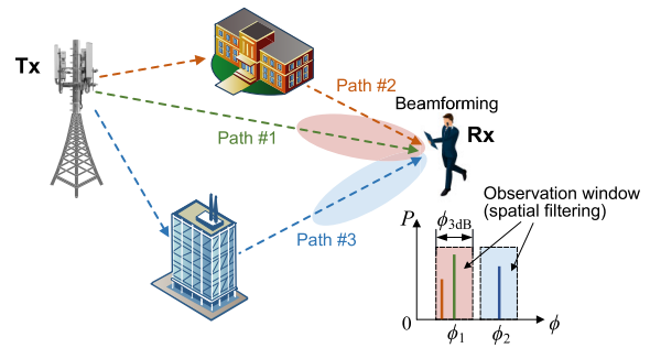
Fig. 1. Illustration of the radio channel observed via specific beam patterns and their impact on channel dispersion.
