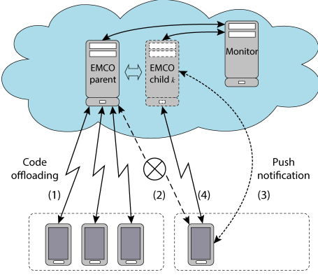
Fig. 6: Multi-tenancy and horizontal scaling in EMCO.
