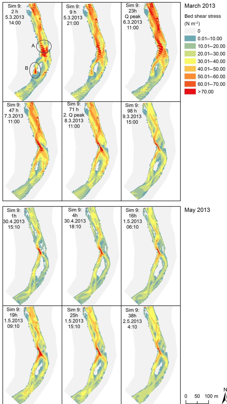
Figure 7. The bed shear stress of simulation 9 during moderate and small discharge events. The key time steps are presented (see Fig. 5).
