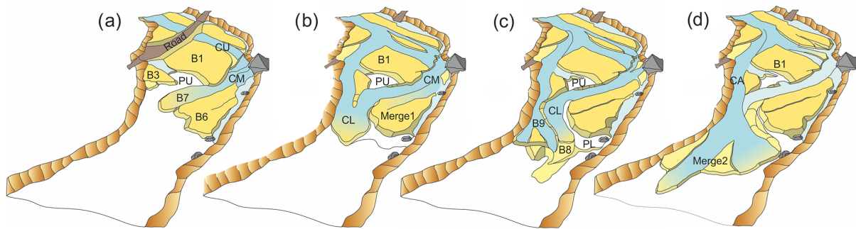
Figure 2. The conceptual graphic presented by Calle et al. (2015: Fig. 10, www.schweizerbart.de/journals/zfg ): the pre-stage of 2012 (a), high flood stage during the March 2013 event (b), low flood stage during the May 2013 event (c), and final stage after May 2013 (d). CU: upper channel; CM: middle channel; CL: lower channel; PU: upper pool; PL: lower pool; B1–9: gravel bars (see Calle et al., 2015).
