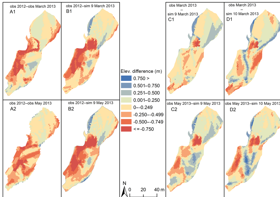
Figure 4. The comparison between the observed and simulated (simulations 9 and 10) elevations. The negative values (red) mean that the observed (A) or simulated (B: simulation 9) March (1) or May (2) 2013 topographies were higher (i.e. deposition had occurred) than was observed in 2012. The negative values also mean that simulated elevations of March or May 2013 were higher than was observed in March or May 2013 with simulations 9 (C) and 10 (D). Simulation 9 corresponded slightly better the observations than simulation 10, and thus its results are shown in more detail. The pool area, in the middle of the area, was the only area where simulation results clearly showed more deposition than observed (see also PU in Fig. 2).
