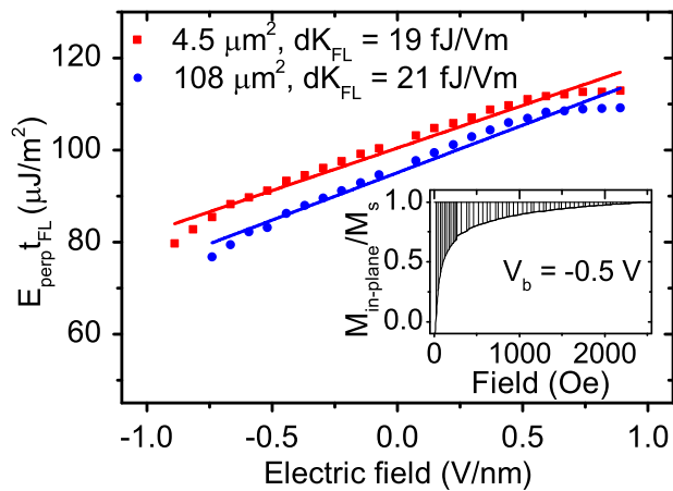
FIG. 4. Perpendicular magnetic anisotropy energy of the CoFeB sensing layer as a function of applied electric field. The data were extracted by integrating M_{in}/M vs. magnetic field curves for MTJs with an area of 4.5 \mu\text{m}^2 and 108 \mu\text{m}^2 (inset).
