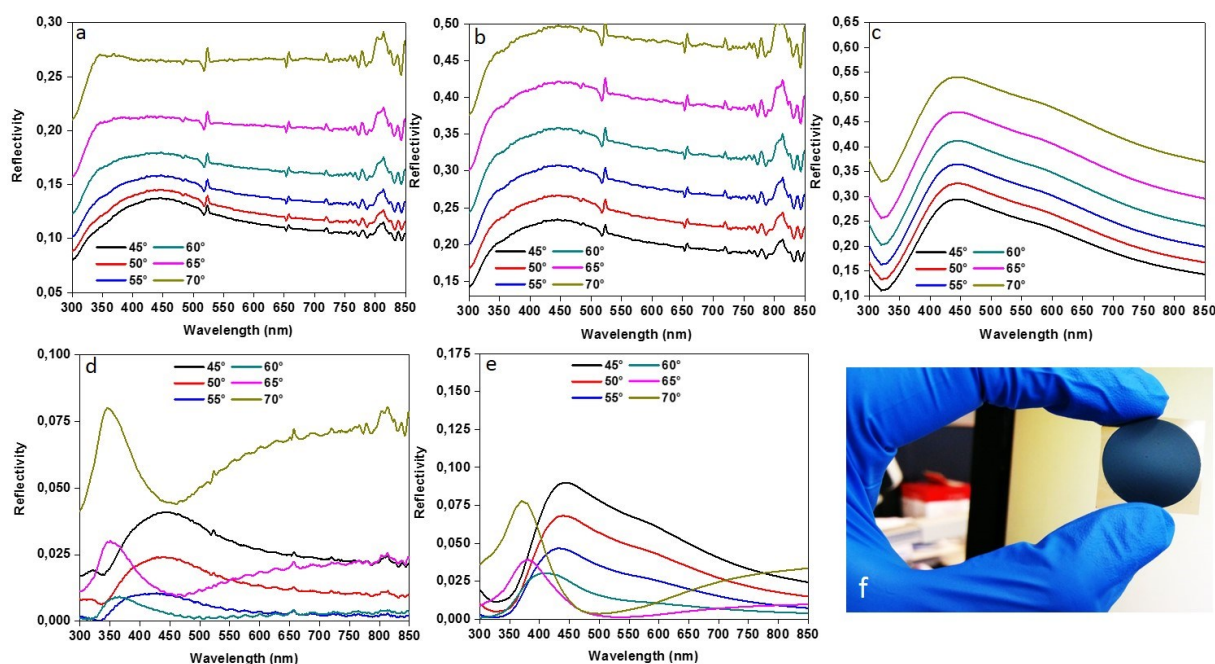
Figure 2. Specular reflection by a plasmonic nanocomposite. a) The total specular reflection spectra of a 20 nm Ag/SiO 2 nanocomposite in various oblique incidence angles. The experimental (b) and simulation (c) based s- polarized specular reflection spectra of the 20 nm Ag/SiO 2 nanocomposite in various oblique incidence angles. The experimental (d) and simulation (e) based p- polarized specular reflection spectra of the 20 nm Ag/SiO 2 nanocomposite in various oblique incidence angles. f) Camera image of a carbon tape coated with a thin layer of the nanocomposite.
