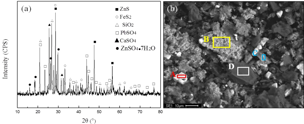
Fig. 4. XRD pattern (a) and EDS image (b) of leaching residues after removing elemental sulfur by washing with CS_2 ( p(O_2) = 0.8 \text{ MPa} , [H_2SO_4] = 180 \text{ g/dm}^3 , t = 2 \text{ h} , T = 159 \text{ }^\circ\text{C} , L/S = 8 \text{ cm}^3/\text{g} )
