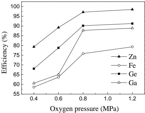
Fig. 3. Effect of oxygen partial pressure on the leaching efficiency of the Zn, Fe, Ge, Ga ( [H_2SO_4] = 180 \text{ g/dm}^3 , t = 2 \text{ h} , T = 159 \text{ }^\circ\text{C} , L/S = 8 \text{ cm}^3/\text{g} )
