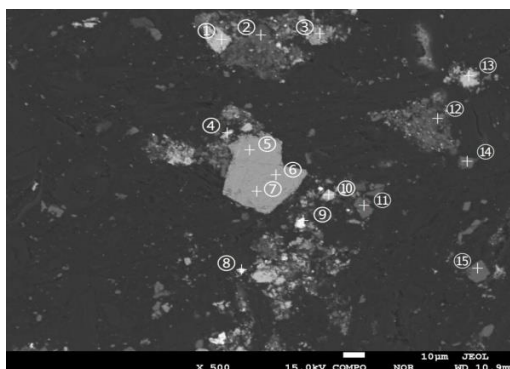
Fig. 9. Backscattered electron image of the leach residues ( p(\text{O}_2) = 0.8 MPa, [\text{H}_2\text{SO}_4] = 180 g/dm 3 , t = 2 h, T = 159 °C, L/S = 8 cm 3 /g, [\text{Cu}^{2+}] = 0.3 g/dm 3 )
