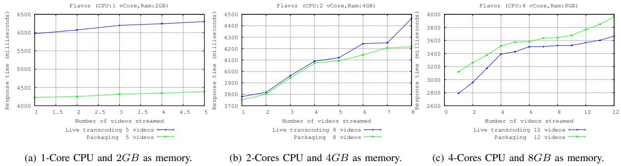
Fig. 5. The response time measured when different flavors are used to instantiate VNFs.
