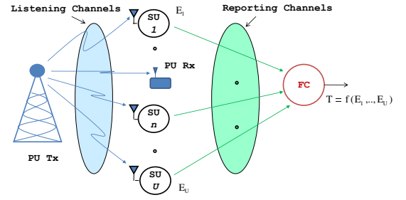
Figure 1. Cooperative energy detection model
