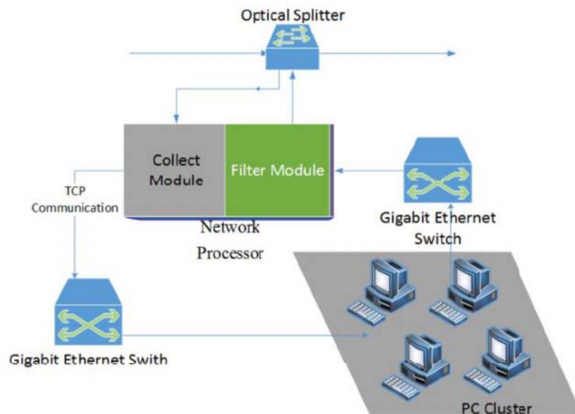
Fig. 3. PC/Network-Processor architecture.
