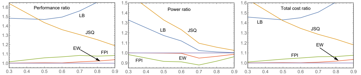
Fig. 1. Ratio of mean number of jobs (left panel), mean power (middle panel) and mean total cost (right panel) to the corresponding quantities of the optimal policy as a function of the load \rho for different policies (LB, JSQ, FPI and EW) with 2 servers.
