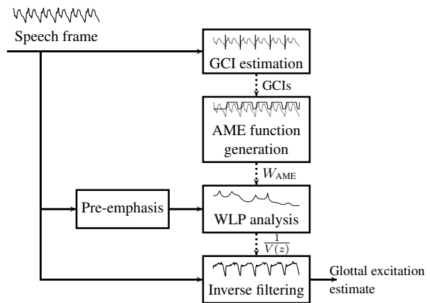
Fig. 1. A block diagram of the QCP glottal inverse filtering method.
