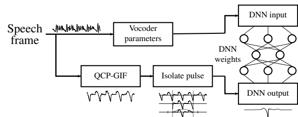
Fig. 3. DNN-based excitation generation framework.
