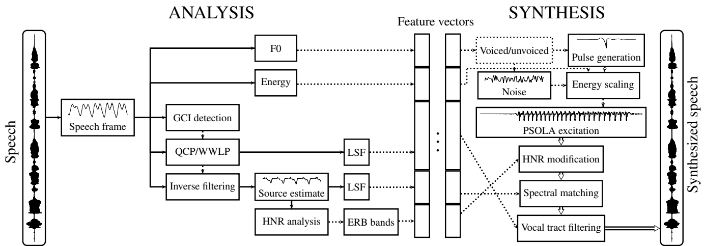
Fig. 2. A block diagram of the GlottDNN vocoder.
