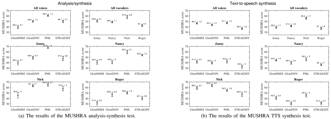
Fig. 6. MUSHRA test results (means and their 95% confidence intervals) obtained with repeated measures ANOVA model ( N = 16 ). For all presented panels the rANOVA p \ll 10^{-3} .
