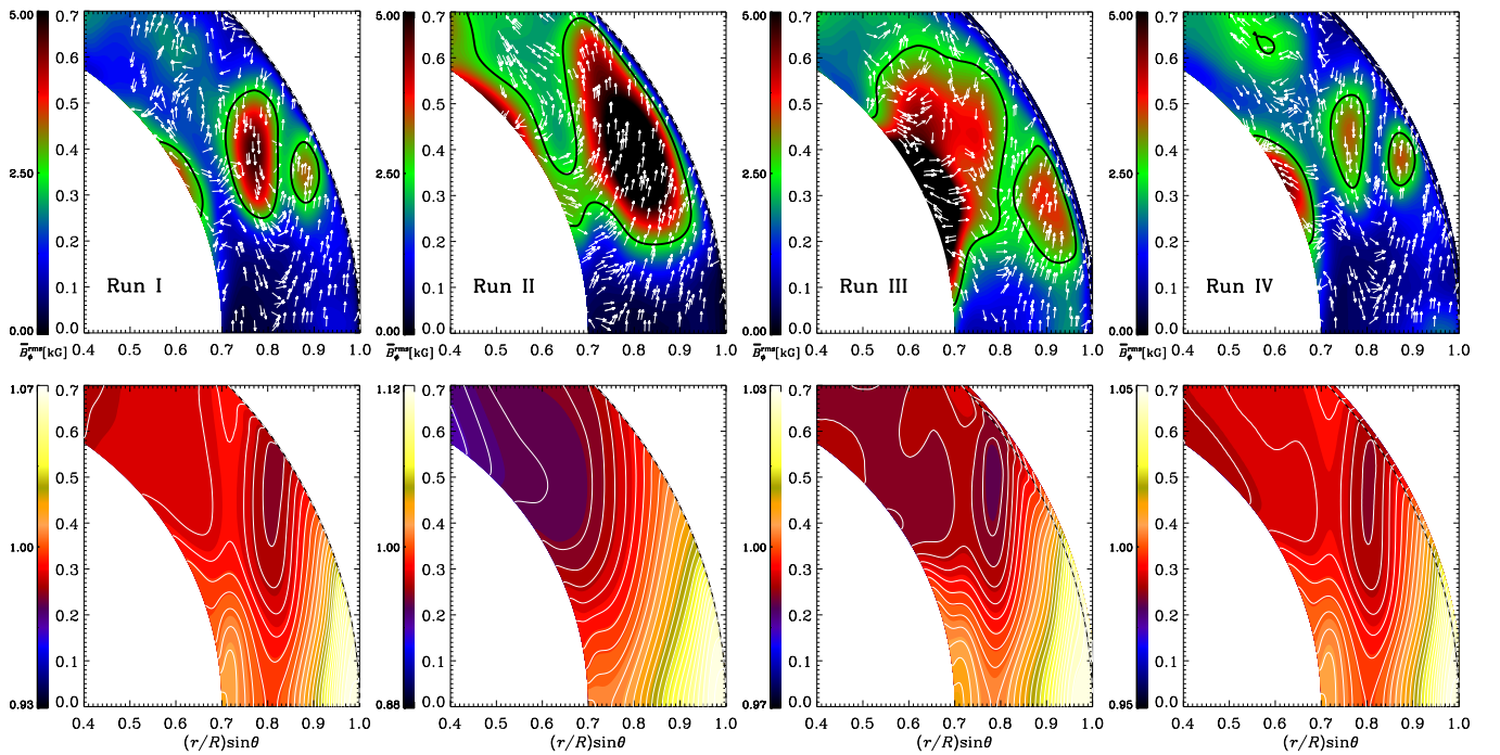
Figure 3. Top row: color coded \bar{B}_\phi^{\text{rms}} during the saturated stage for Runs I–IV (left to right). White arrows show the direction of migration \xi_{\text{mig}}(r, \theta) = -\alpha \hat{e}_\phi \times \nabla \Omega ; see Equation (3). The black solid lines indicate isocontours of \bar{B}_\phi at 2.5 kG. Bottom row: \Omega(r, \theta)/\Omega_0 for the same runs. The dashed lines indicate the surface ( r = R ). (A color version of this figure is available in the online journal.)
