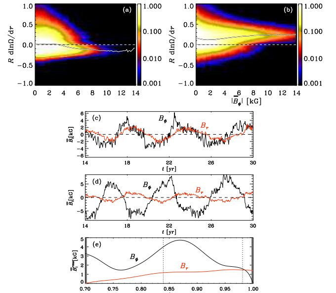
Figure 5. Panels (a) and (b): correlation of |\bar{B}_\phi| from the latitudinal band \pm 15^\circ - \pm 40^\circ and the logarithmic gradient of \Omega for Runs I (a) and II (b). Overplotted are the mean (white) and the zero lines (white-black dashed). (c) and (d): phase relation between \bar{B}_\phi (black) and \bar{B}_r (red) at 25^\circ latitude and r = 0.98 R (c) and at r = 0.84 R (d) for Run I. (e): Time-averaged radial dependence of \bar{B}_\phi^{\text{rms}} (black) and \bar{B}_r^{\text{rms}} (red) at 25^\circ latitude for Run I.
