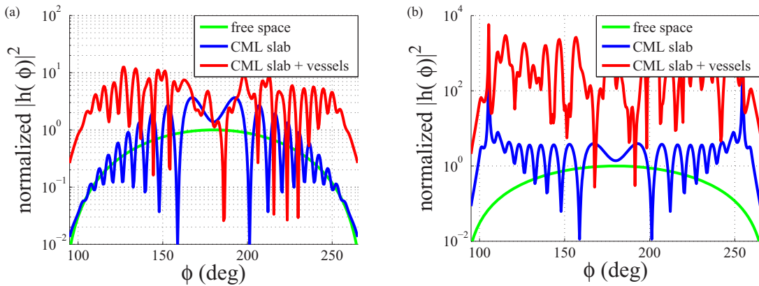
FIG. 10. The azimuthal profiles |h(\varphi)|^2 (normalized by |h_{\text{inc}}(0)|^2 = k_0^2 \omega^2 q^2 / 16 ) of the incident field, the background field and the total field as functions of angle \varphi for: (a) a passive scenario ( \delta = +0.01 ) and (b) an active scenario ( \delta = -0.01 ). Plot parameters: a = -2 , b = 0 , L = 3\lambda_0 , g\lambda_0/10 , r = \lambda_0/100 , N = 80 , \theta = 90^\circ .
