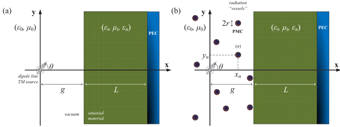
FIG. 1. (a) The testbed configuration of a grounded electrically thick slab filled with a uniaxial material (\epsilon_t, \mu_t, \epsilon_n) with the thickness L , excited by a TM electric dipole line inclined by the angle \theta located at a small distance g from the air-medium interface. (b) The same structure in the presence of a cluster of N electrically thin (the radius r ) circular perfect magnetic conductor (PMC) cylinders randomly distributed in the vicinity of the air-slab interface with arbitrary coordinates (x_n, y_n) for n = 1, \dots, N .
