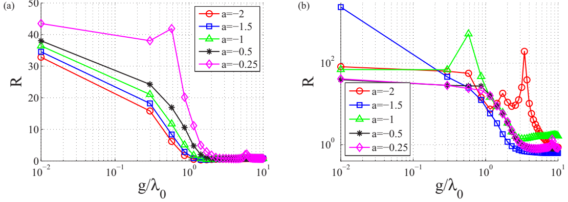
FIG. 9. The radiation enhancement ratio R for various values of the real part of transversal components a = \text{Re}[\epsilon_t] = \text{Re}[\mu_t] as a function of the electrical distance of the source from the interface g/\lambda_0 ( L = 3\lambda_0 ). (a) Overall passive CML with \delta = 0.02 . (b) Overall active CML with \delta = -0.02 . Plot parameters: b = 0.2 , r = \lambda_0/200 , N = 80 , \theta = 90^\circ .
