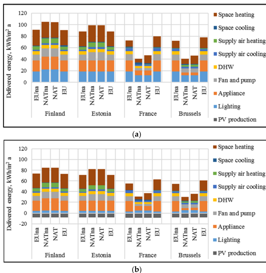
Figure 8. Comparison of delivered energy use in simulated cases with reference and national input values. (a) 2016. (b) NZEB. PV production refers as onsite electricity production from the photovoltaic panel (PV).
