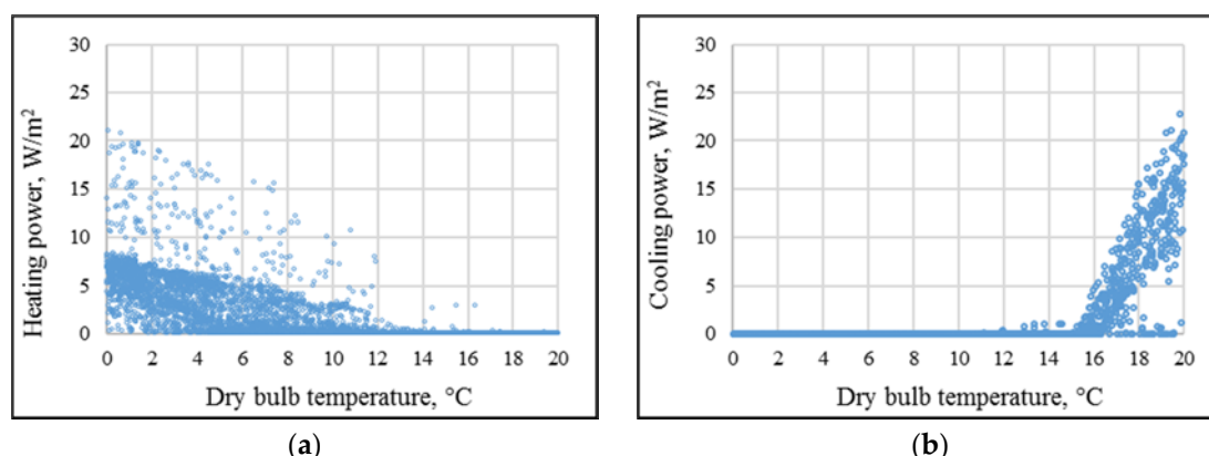
Figure 4. Base temperature selection for reference office building 2016 in Estonian climate (a) space heating and (b) cooling.
