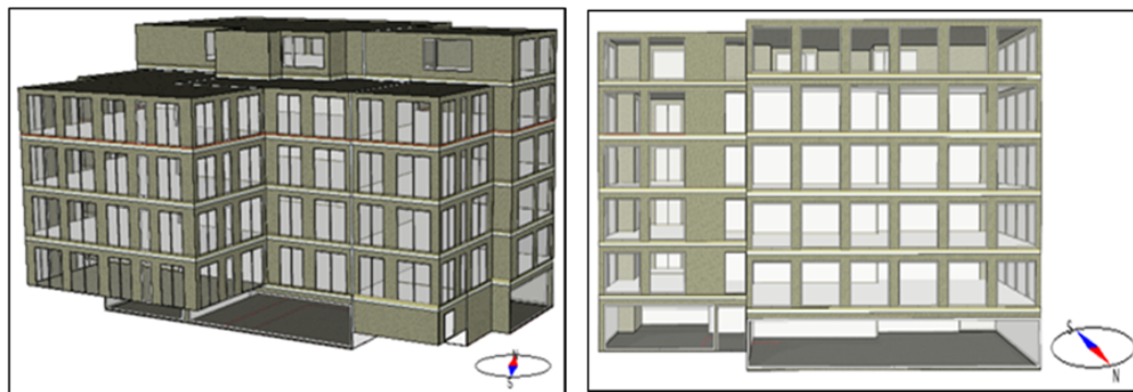
Figure 3. 3D model of simulated reference office building. Figure 3. 3D model of simulated reference office building.
