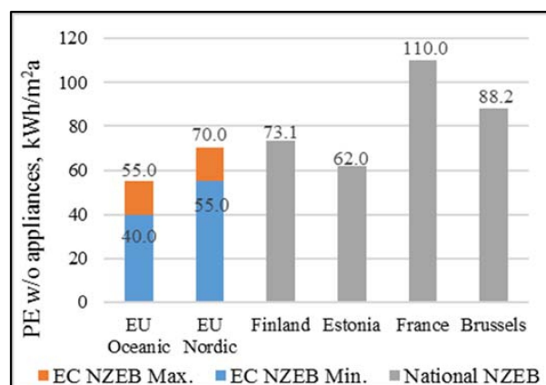
Figure 2. The compliance of national NZEB requirements with EC recommendations, a direct comparison without taking into account national input data and primary energy factors differences.
