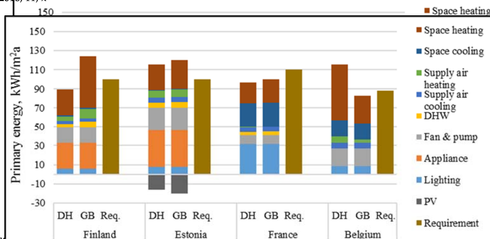
Figure 10. Primary energy in NZEB office buildings with changed parameters in order to target NZEB requirements.
