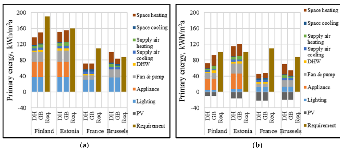
Figure 9. Primary energy in NAT cases office buildings compared with regulation (a) 2016, (b) 2021 NZEB.
