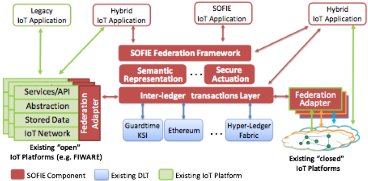
Figure 1: Overview of the SOFIE federation architecture, its components and relationships to existing systems
