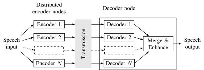
Fig. 3. Encoder/decoder structure of the distributed speech and audio codec with N encoder nodes and a single decoder node.
