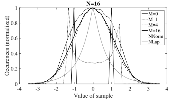
Fig. 5. Normalized histograms of the output samples after M consecutive randomizations, as well as the theoretical distributions of normalized Gaussian ( NNorm , dashed line) and Laplacian ( NLap , gray line), for a vector of length N = 16 .
