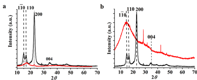
Figure 4. XRD of native CNCs (black curves) (a,b), cellulose 2H,2H,3H,3H-perfluorononanoyl ester before the nanoprecipitation dropping technique (red curve) (a) and NPs of the cellulose 2H,2H,3H,3H-perfluorononanoyl ester after the nanoprecipitation dropping technique (red curves) (b).
