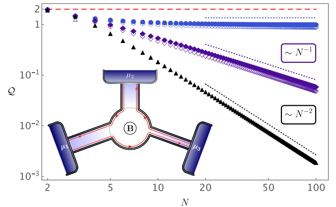
FIG. 1. Uncertainty products Q for ballistic multiterminal transport as a function of N . Inset: Setup for N = 3 , with currents flowing along quantum Hall edge states (red lines). Main figure: Both Q_N for the most precise basis current (blue circles: full LR, empty beyond), and Q_{\text{lin}} for the optimal current (purple diamonds: full LR, empty beyond) for linear bias profile break the time-reversible TUR (1) (red dashed line). Q_{\text{sin}} for sinusoidal bias (black triangles: full LR, empty beyond) saturates the LR bound (13).
