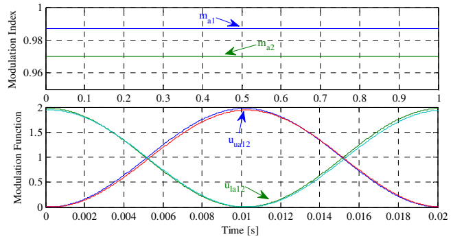
Fig. 3. The designed modulation index and function according to the new parameters of Table II.
