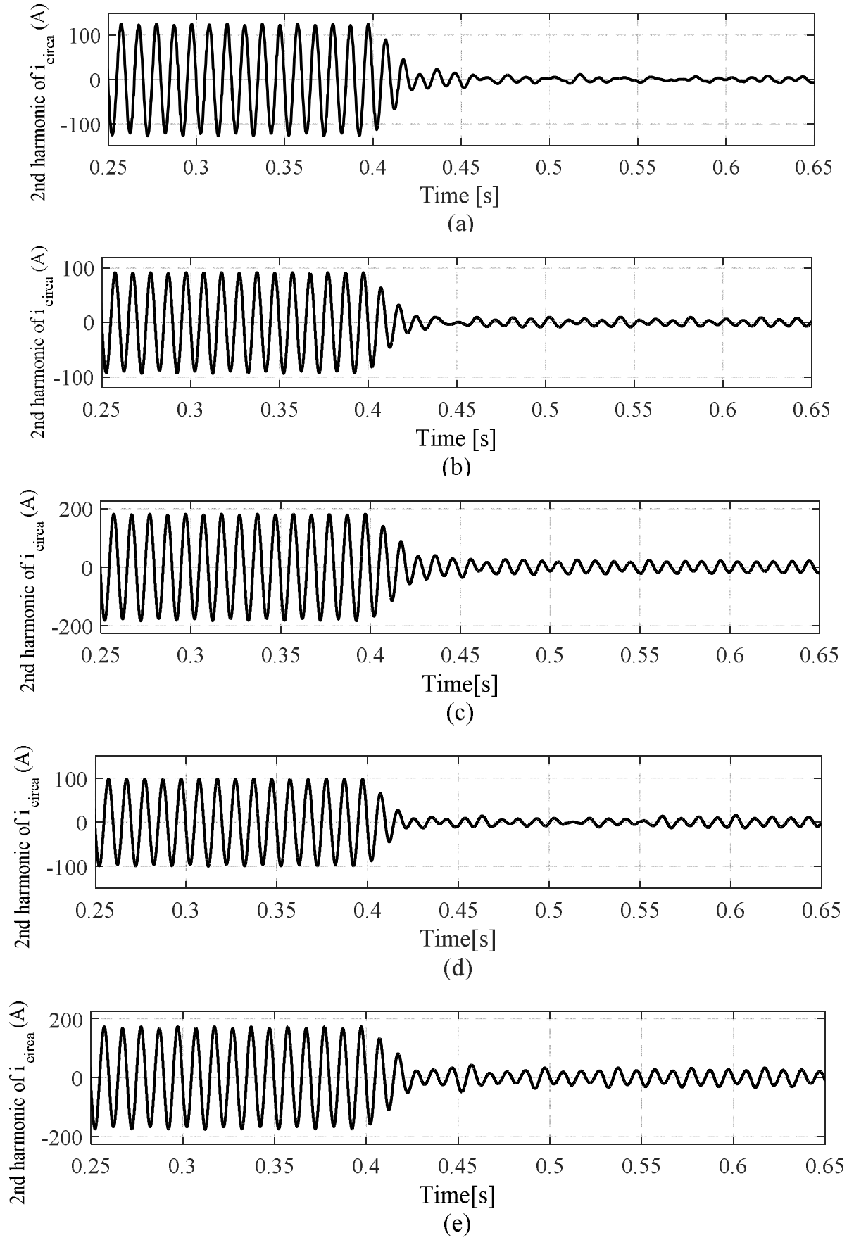
Fig. 10. Simulation results for second harmonic component of i_{circa} , (a) L_{arm}=9\text{mH} and C_{SM}=10\text{mF} , (b) L_{arm}=1.2\times 9\text{mH} and C_{SM}=10\text{mF} , (c) L_{arm}=0.8\times 9\text{mH} and C_{SM}=10\text{mF} , (d) L_{arm}=9\text{mH} and C_{SM}=1.2\times 10\text{mF} , (e) L_{arm}=9\text{mH} and C_{SM}=0.8\times 10\text{mF} .
