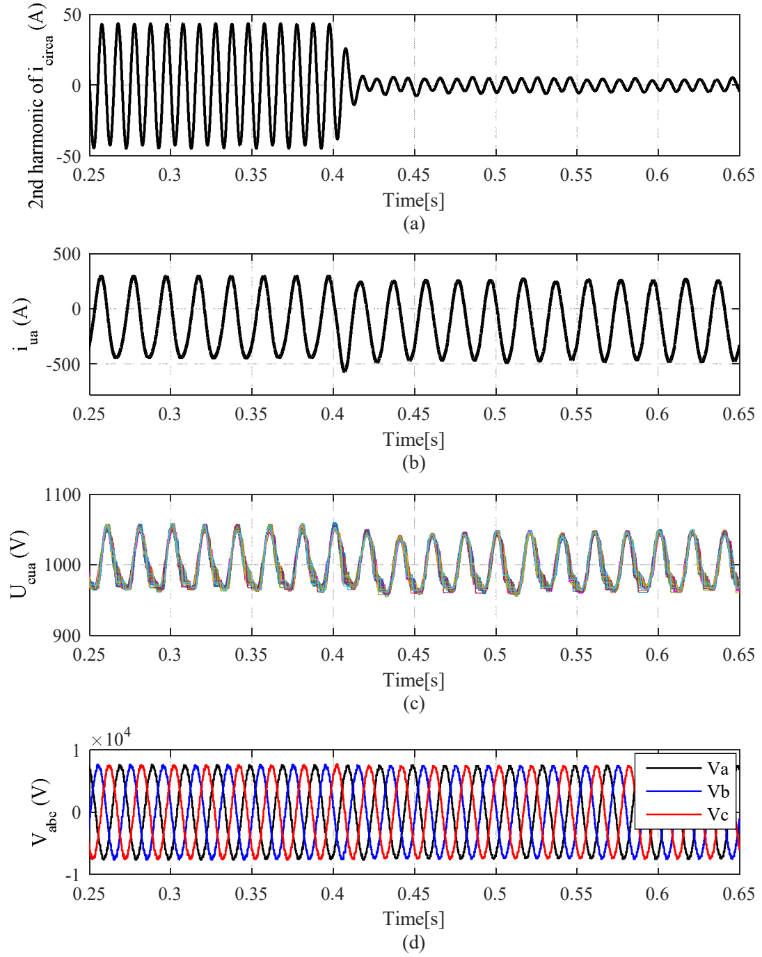
Fig. 8. Simulated waveforms of the MMC with 20% increase in all L_{arm} , L_c , and C component values:
