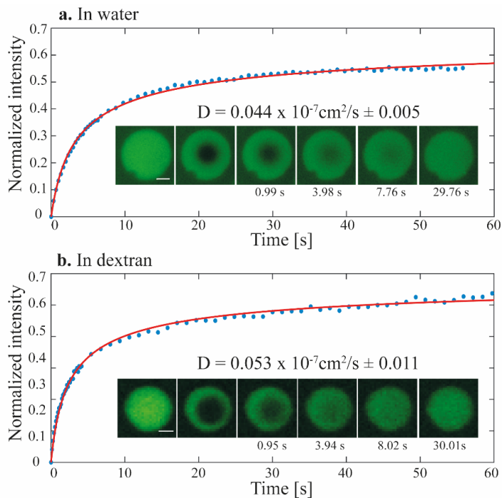
Fig. 6. FRAP recovery of partially bleached CBM-eDAF3-CBM coacervate (a) in water, scale bar 2 \mu\text{m} , and (b) in 10 % dextran, scale bar 4 \mu\text{m} . The time scale of images is in seconds after the bleach. Diffusion is presented as a mean value \pm std ( n = 5 ).
