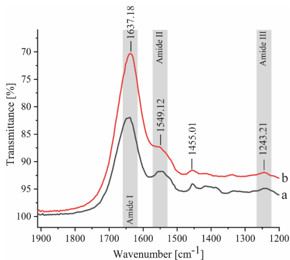
Fig. 7. FTIR spectra of CBM-eADF3-CBM in water (a) and in the presence of 50 \text{gl}^{-1} dextran (b).
