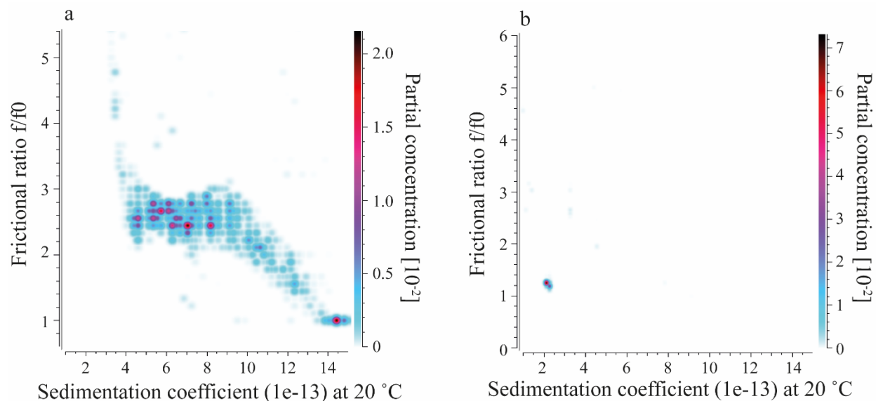
Fig. 3. (a) Pseudo 3D plot of pure dextran measured at 660 nm displaying a wide distribution of dextran with higher f/f_0 and S values. (b) Pseudo 3D plot of CBM-dextran mixture measured at 280 nm. A CBM peak is observed at S = 2.15 \cdot 10^{-13} , f/f_0 = 1.2 . Dextran is invisible at 280 nm. However, in the case of interaction between CBM and dextran, the latter would cause changes in the distribution of CBM.
