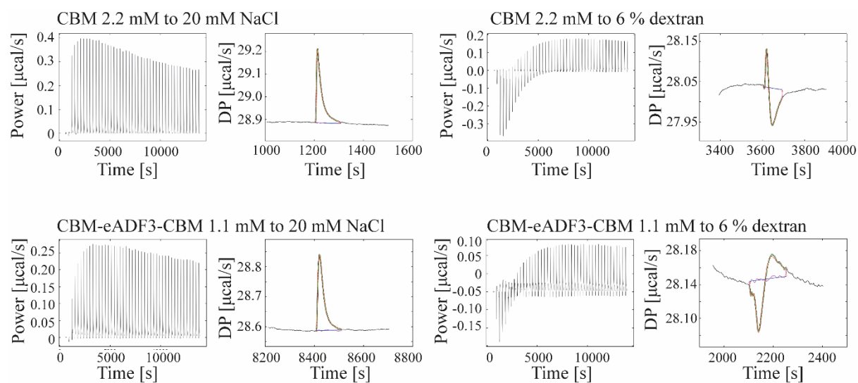
Fig. 2. Representative data from ITC experiments and magnification of the peak shape.
