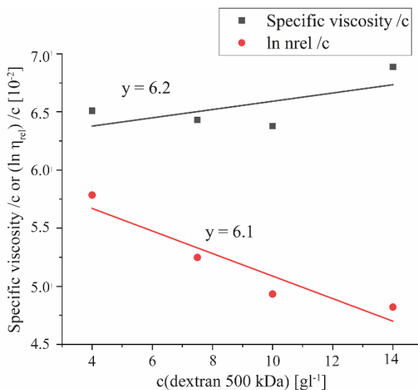
Fig. 8. Huggins ( \eta_{sp}/c vs. c ) and Kraemer ( (\ln \eta_{rel})/c vs. c ) plot of dextran 500 kDa.
