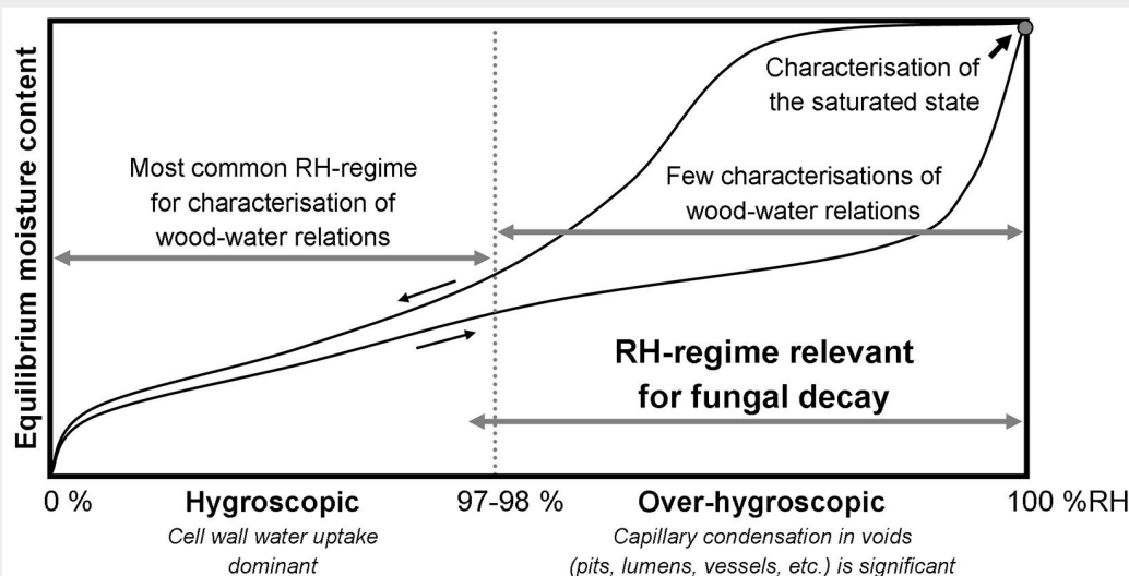
Fig. 1 - Schematic illustration of sorption isotherms for wood in absorption from absolute dry state (lower black line) and desorption from fully water-saturated state (upper black line) in the entire relative humidity (RH) range.
