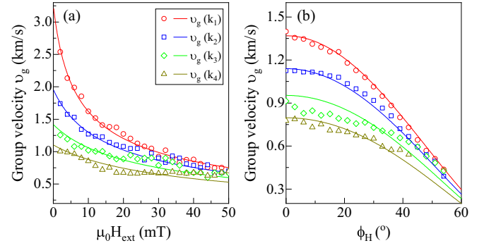
FIG. 7. Spin-wave group velocity v_g of k_1 – k_4 modes as a function of (a) external magnetic bias field and (b) field angle. In (a) \phi_H = 0^\circ , and in (b) \mu_0 H_{\text{ext}} = 15.5 mT. The symbols and colored lines represent experimentally derived values and calculations using Eq. (6).
