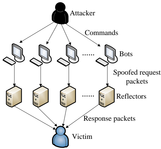
Fig. 6. DRDoS flooding attacks
