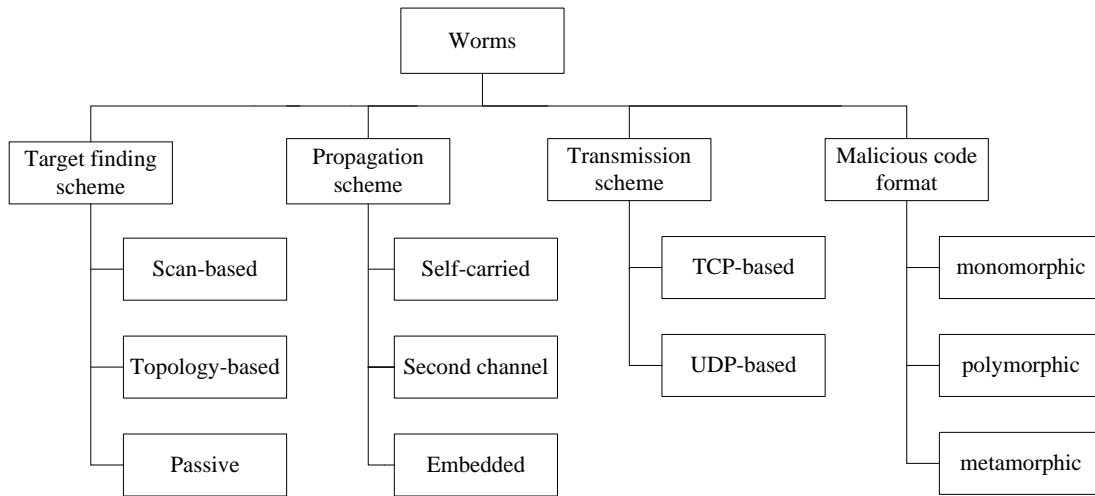
Fig. 8. The classification of worm characteristics
