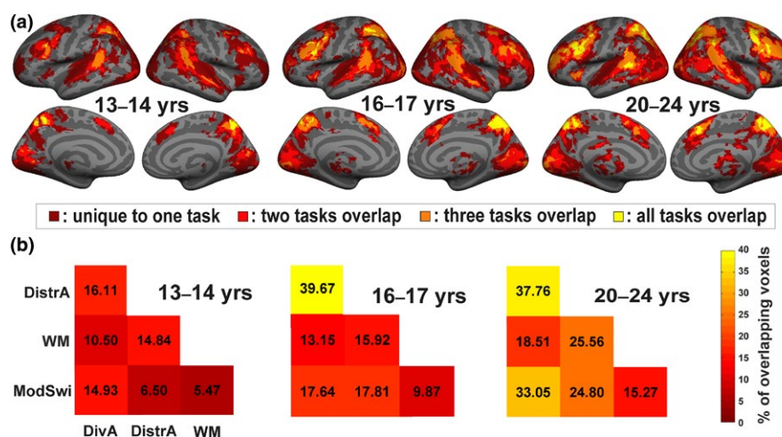
FIGURE 3 (a) Voxels showing significant activity enhancements ( t > 2.7 , k > 250 , cluster-level FWE-corrected p < 0.01 ) in response to one or more of the executive tasks, with the color of the voxel denoting how many of the executive tasks significantly activate that voxel. Dark red regions: activity enhancements for only one executive task, bright red regions: two executive tasks overlap, orange: three executive tasks overlap, yellow: all four executive tasks overlap. The maps are plotted for each age cohort separately. (b) The percentage of overlapping, significantly activated voxels between each of the executive task types is visualized in a matrix for each age cohort separately. DivA: Divided attention; DistrA: Distracted attention; ModSwi: Modality switch; WM: Working memory
