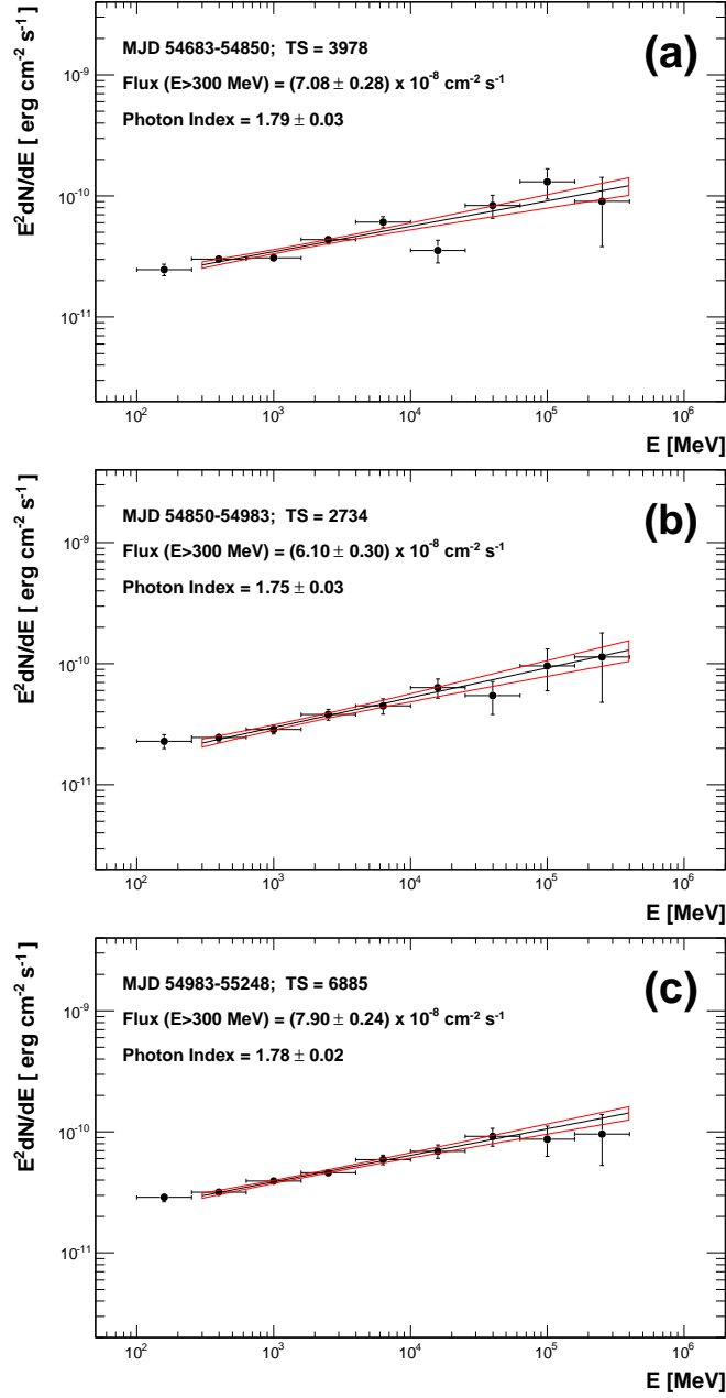
Fig. 7.— Fermi spectra of Mrk 421 for several time intervals of interest. The panel (a) shows the spectrum for the time period before the multifrequency campaign (MJD 54683-54850), the panel (b) for the time interval corresponding to the multifrequency campaign (MJD 54850-54983) and the panel (c) for the period after the campaign (MJD 54983-55248). In all panels, the black line depicts the result of the unbinned likelihood PL fit and the red contours denote the 68% uncertainty of the PL fit. The legend reports the results from the unbinned likelihood PL fit in the energy range 0.3 – 400 GeV.
