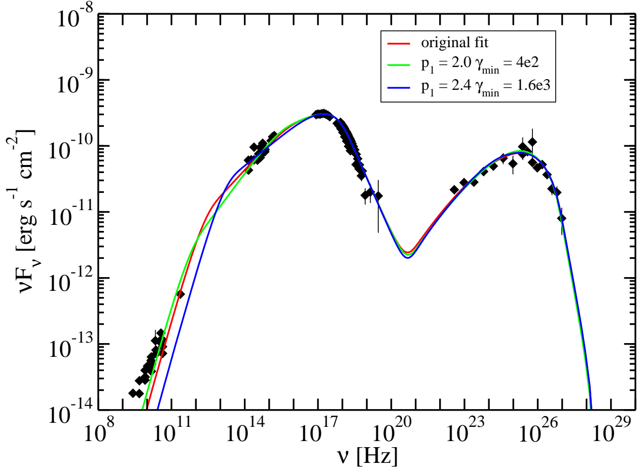
Fig. 12.— SSC model fit of the SED from Mrk 421 presented in Figure 11 (for t_{var} \sim 1 day), with variations by a factor of 2 of the parameter \gamma_{min} , together with adjustments in the parameter p_1 in order to match the experimental data. See text for further details.
