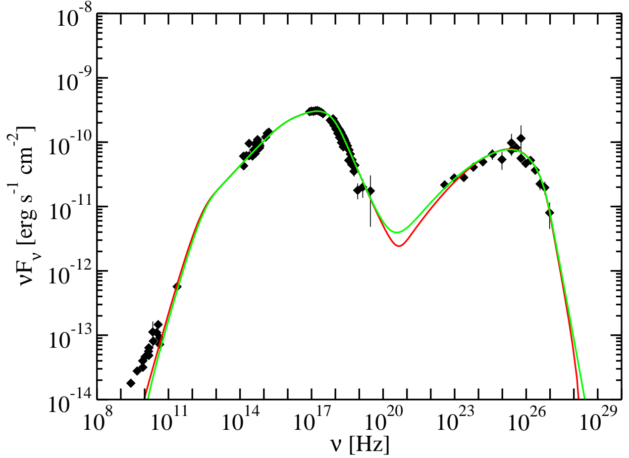
Fig. 11.— SED of Mrk 421 with two 1-zone SSC model fits obtained with different minimum variability timescales: t_{var} = 1 day (red curve) and t_{var} = 1 hour (green curve) . The parameter values are reported in Table 4. See text for further details.
