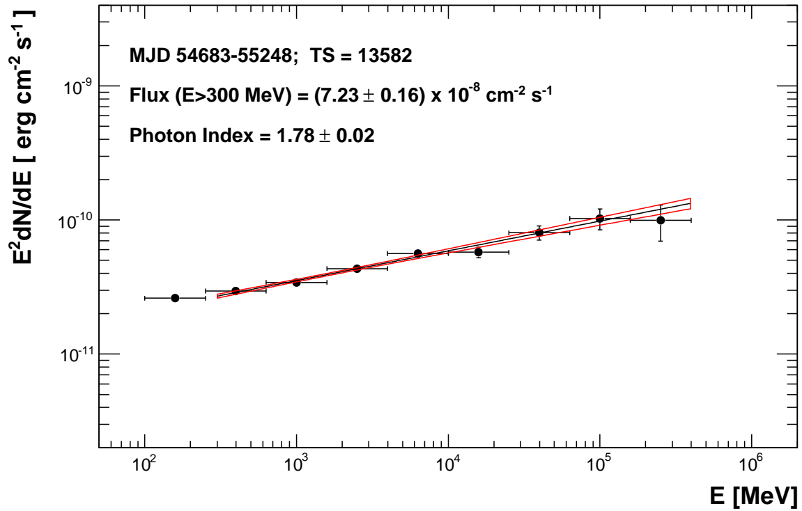
Fig. 5.— Fermi spectrum of Mrk 421 during the period from 2008 August 5 to 2010 February 20. Black line is the likelihood PL fit; red contour is the 68% uncertainty of the fit and the black data points show the energy fluxes computed on differential energy ranges. The inlay summarizes the unbinned likelihood PL fit in the energy range 0.3-400 GeV.
