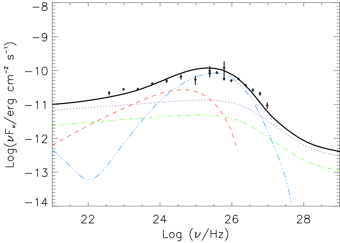
Fig. 10.— Expanded view of the high energy bump of the SED data and model presented in Figure 9.
