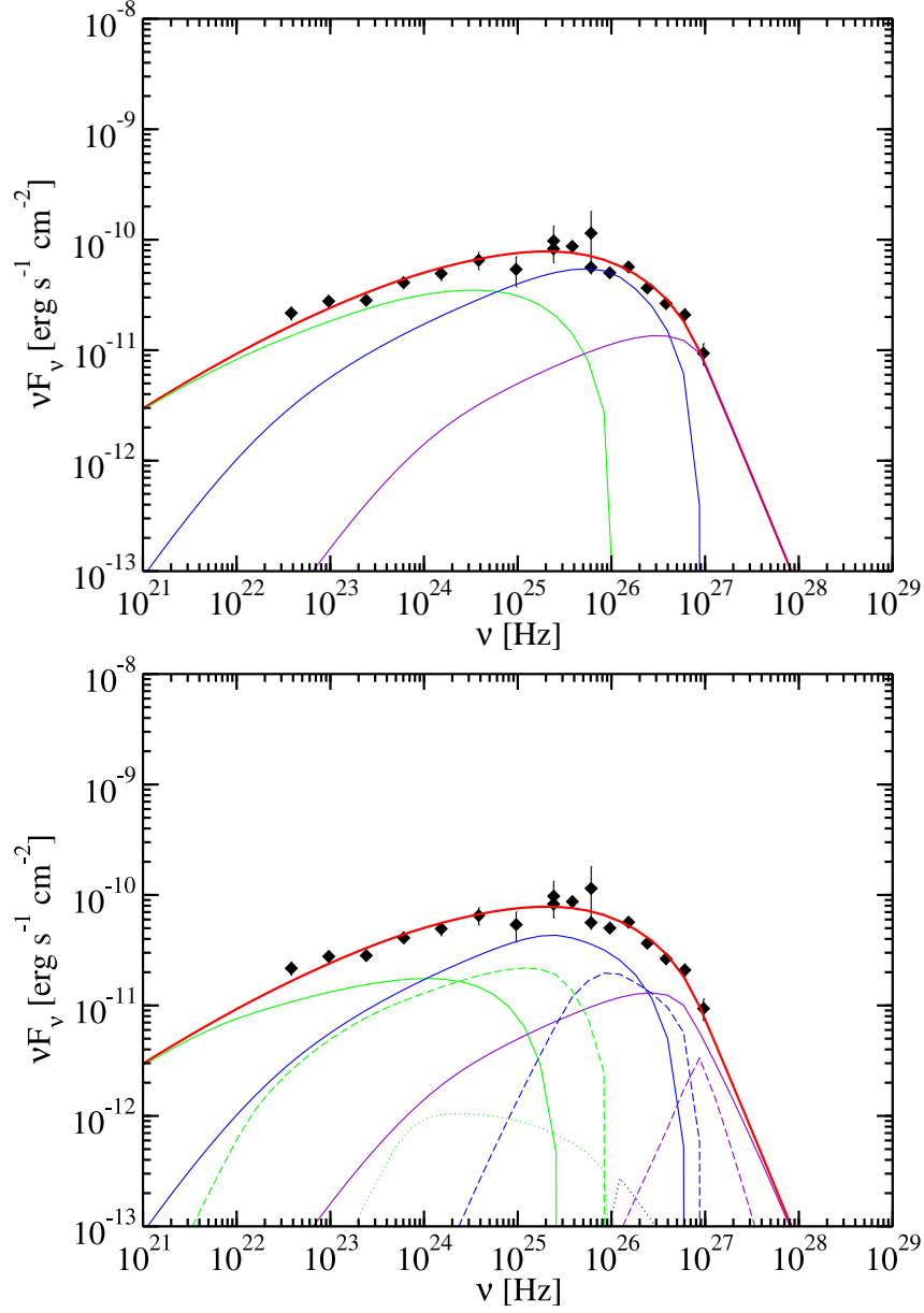
Fig. 13.— Decomposition of the high energy bump of the SSC continuum for Mrk 421. The data points are the same as in the high energy bump from Figure 11. The SSC fit to the average spectrum is denoted by the red solid curve. Top: Contributions of the different segments of electrons comptonizing the whole synchrotron continuum (green curve: \gamma_{min} < \gamma < \gamma_{br,1} ; blue curve: \gamma_{br,1} < \gamma < \gamma_{br,2} ; purple curve: \gamma_{br,2} < \gamma ). Bottom: Contributions of the different segments of electrons (as in the top panel) Comptonizing different segments of the synchrotron continuum (solid curves: \nu < \nu_{br,1} \simeq 5.3 \times 10^{15} Hz; dashed curves: \nu_{br,1} < \nu < \nu_{br,2} \simeq 1.3 \times 10^{17} Hz; dotted curves, corresponding to \nu > \nu_{br,2} )
