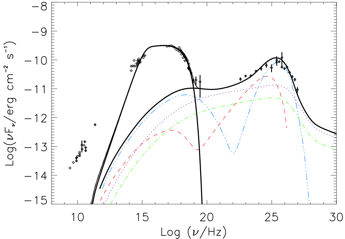
Fig. 9.— Hadronic model fit components: \pi^0 -cascade (black dotted line), \pi^\pm cascade (green dashed-dotted line), \mu -synchrotron and cascade (blue dashed-triple-dotted line), proton synchrotron and cascade (red dashed line). The black thick solid line is the sum of all emission components (which also includes the synchrotron emission of the primary electrons at optical/X-ray frequencies). The resulting model parameters are reported in table 3.
