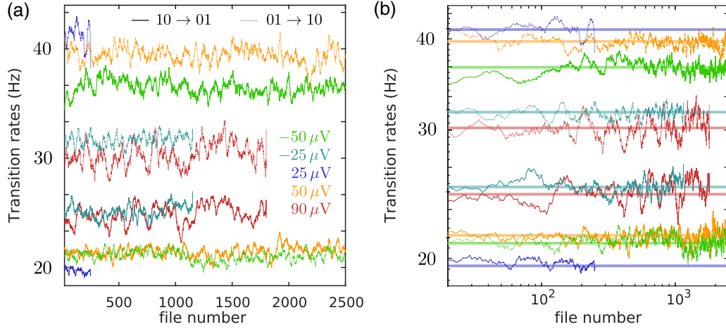
FIG. 3. Fluctuations in transition rates over time. The transition rates \Gamma_{(1,0), (0,1)} (solid lines) and \Gamma_{(0,1), (1,0)} (dotted lines) as a function of file numbers for different bias voltages [see legend in (a)]. Each file is a 15-s time evolution of system charge state. The transition rates are evaluated using Eq. (D1) (as described in Sec. II and Appendix D) and the variables N_{n \rightarrow n'} , P^{\text{st}}(n) computed for the individual files with time duration \tau = 15 s. The solid line in (b) is the average transition rate (shown in Table I) used for computing the entropy production using Eqs. (1)–(4).
