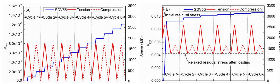
Fig. 11. Stress and p_{acc} variation with fatigue cycles: (a) without residual stress; (b) with residual stress.
