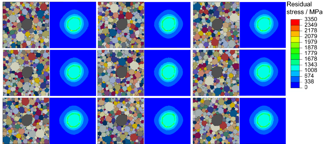
Fig. 8. Nine different RVEs of virtual martensitic microstructure with the same geometry of the inclusion shown in Fig. 5(a) in the centre and the corresponding residual stress distributions after the cooling simulation.
