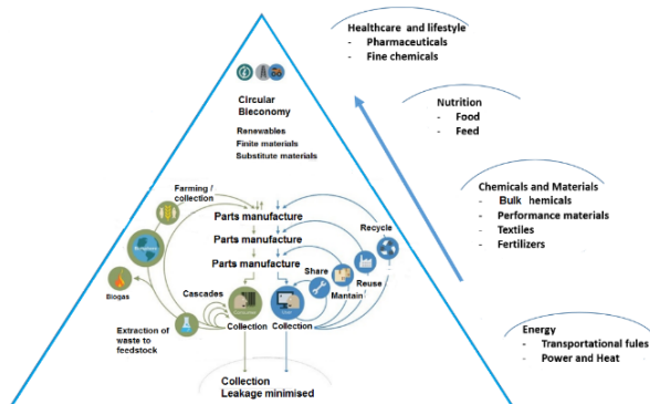
Fig. 4 Schematic illustration of closed loop concept of bioeconomy with cascading concept within the bio-mass values pyramid /adopted from references / [3,14,24] /
