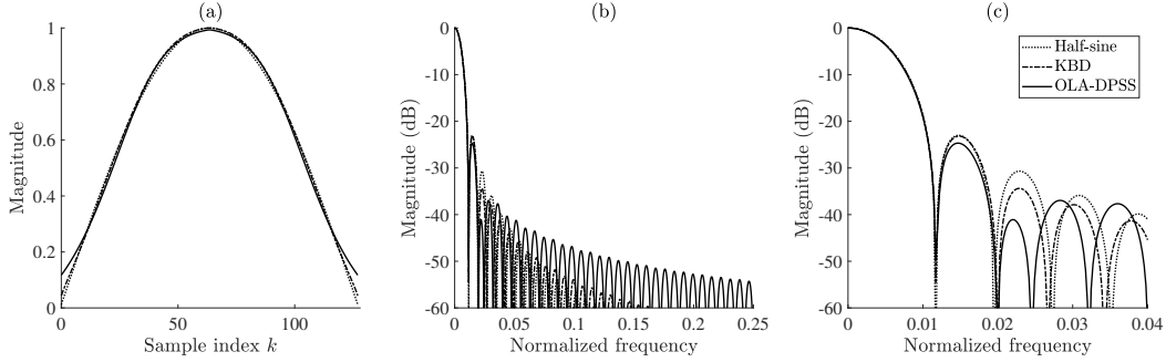
Fig. 5. Illustration of (a) the half-sine, KBD and proposed OLA-DPSS windows, (b) their spectral responses and (c) responses focused on the central region. Window length is L = 128 and KBD has \alpha = 4.25 and OLA-DPSS has \alpha = 2.75 .
