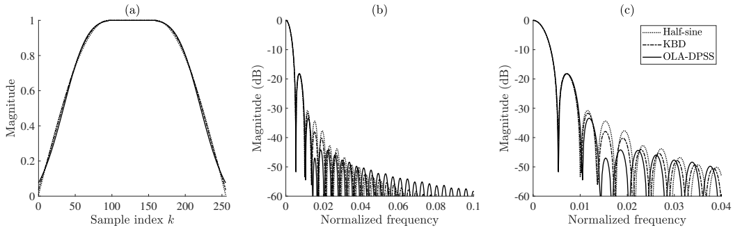
Fig. 6. Illustration of low-overlap versions of (a) the half-sine, KBD and proposed OLA-DPSS windows, (b) their spectral responses and (c) responses focused on the central region. Window length is L = 256 , overlap length is T = 64 , KBD has \alpha = 4.25 and OLA-DPSS has \alpha = 5 .
