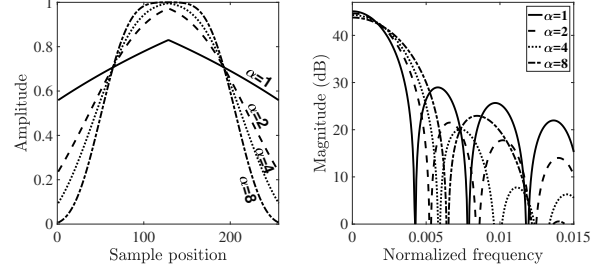
Fig. 4. Illustration of the shapes of proposed window with different values of \alpha and a window length of L = 256 .
