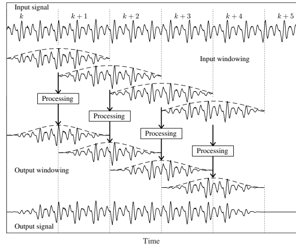
Fig. 1. Illustration of input and output windowing with overlap-add synthesis in a speech processing application.
