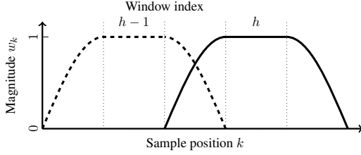
Fig. 3. To obtain a low overlap between windows, we can constrain a number of samples in the middle of the window to have unit magnitude. Thin dotted vertical lines indicate the borders between the flat tops and overlap areas.
