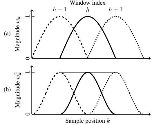
Fig. 2. (a) Typical input windowing functions of subsequent frames and (b) the corresponding squared windowing functions. The thin line in (b) demonstrates the region where the windows add up to unity as required by Eq. 4.
