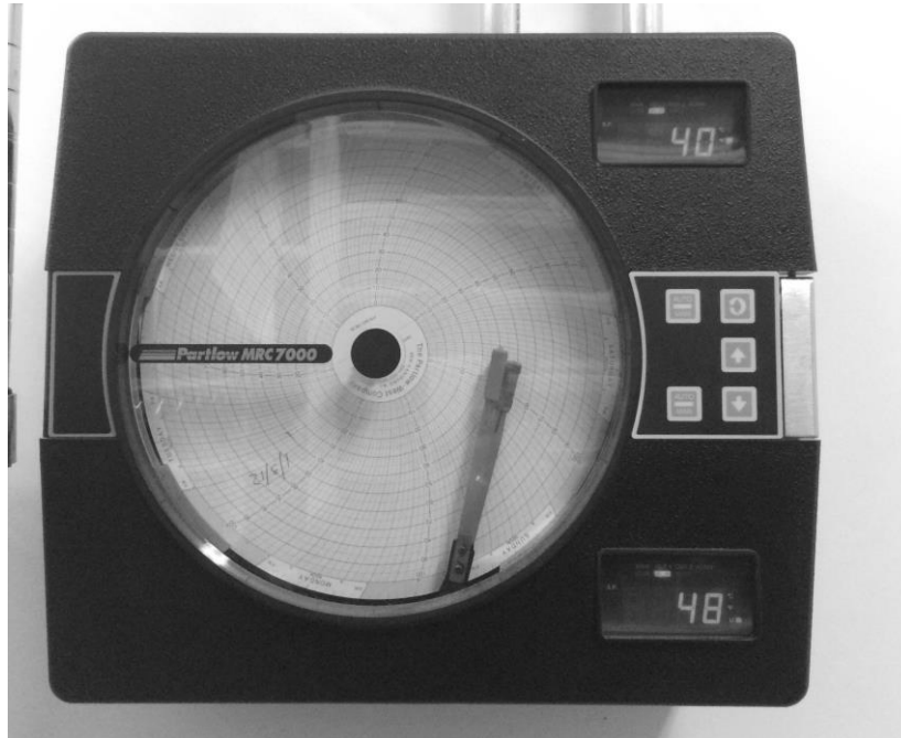
Fig. 3. The Circular Chart Recorder at the Crozier Storage and Conservation Facility of the Cooper Hewitt Smithsonian Design Museum records temperature and humidity measurements on a round chart over a timed interval. Image by Samir Bhowmik.
