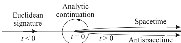
Fig. 1. Bifurcation at Big Bang. Analytic continuation in physical proper time t : the scale factor a(t) \propto \sqrt{t} changes sign around the Big Bang point, transforming spacetime into antispacetime. At t < 0 the scale factor is imaginary, which corresponds to the metric with Euclidean signature. Crossing the Big Bang from the t < 0 semiaxis, the Universe approaches either spacetime or antispacetime. In this scenario, the Big Bang represents the bifurcation point at which the Z_2 symmetry between the spacetime and antispacetime is spontaneously broken. The quantum superposition of the two states is not allowed in the macroscopic system
