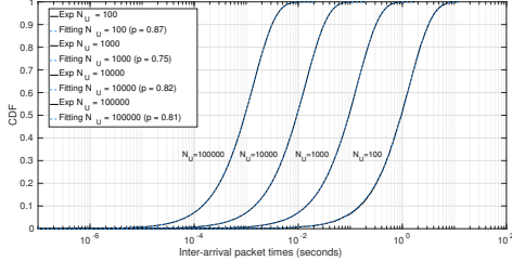
Fig. 9: CDF of the inter-arrival signaling procedures for a population density of 500 habs/km².
