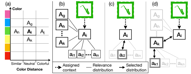
Figure 2: The mood board is best described by strategy A_i . (a) Simplified 2D context space with possible strategies. (b) A_i selects the best relevance probability, either (c) one of its suggestion agents a_{in} or (d) one of its neighboring strategies A_{e..m} , which queries its own suggestion agents. Selected distributions are individually updated based on feedback.
