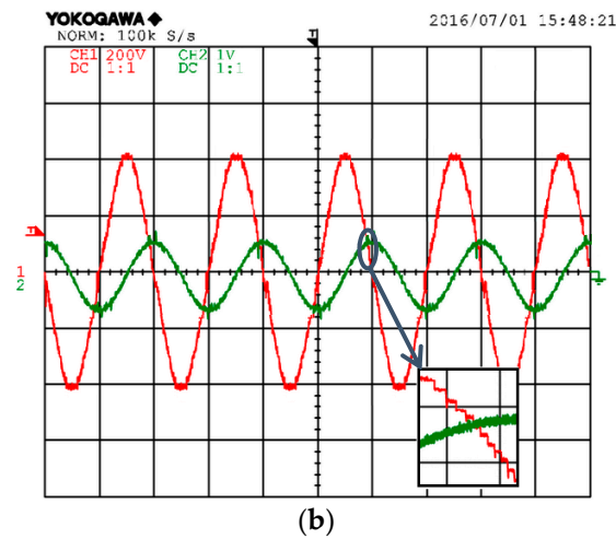
Figure 12. Experimental results (a) Test set up (volt/div = 200 volts), (b) Output voltage and current in pure inductive load (Ampere/div = 1 amps) (time/div = 2500 \mu s).
