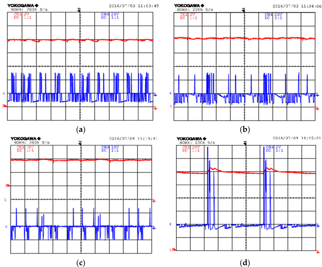
Figure 13. Voltage and current of capacitors (all channels time/div = 2500 \mu s) (a) C_{M1} (volt/div = 2 volts, Ampere/div = 20 amps), (b) C_{M2} (volt/div = 2 volts, Ampere/div = 20 amps), (c) C_{M3} (volt/div = 10 volts, Ampere/div = 10 amps), (d) C_{M7} (volt/div = 20 volts, Ampere/div = 2 amps).
