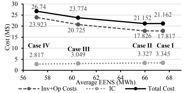
Fig. 2. Various cost terms versus average EENS in different Cases.
