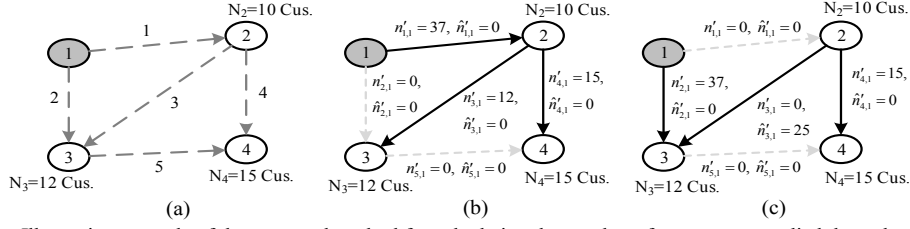
Fig. 1. An Illustrative example of the proposed method for calculating the number of customers supplied through each line.
