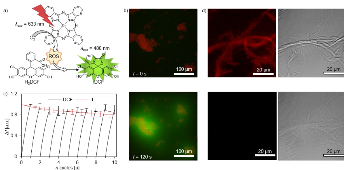
Figure 5. (a) Schematic representation of the photoinduced oxidation process. Absorption of red light ( \lambda_{\text{exc}} = 633 \text{ nm} ) by the chromophore induces the excitation of molecular oxygen present in the media to ROS, which oxidizes the precursor ( \text{H}_2\text{DCF} , non-fluorescent) into DCF ( \lambda_{\text{exc}} = 488 \text{ nm} ). Note that the peripheral substituents of 1 has been omitted for clarity purposes. (b) Time-lapsed emission microscopy images of the bundled fibers (red) and in-situ photooxidized DCF (green). \text{H}_2\text{DCF} is present at 750 \mu\text{M} in acetate buffer (10 mM pH = 5.5). (c) Averaged and normalized increase of DCF (black) and decrease of 1 (red) after 2 min irradiation (60 frames) per cycle. Error bars correspond to the standard deviation of three bundles. Normalized data to the end value of the first cycle (DCF) and the initial emission 1 . (d) Emission ( left ) and bright field ( right ) micrographs of fibers before ( top ) and after
