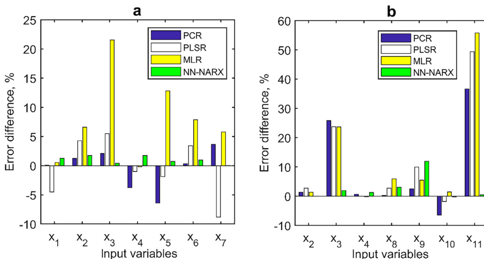
Fig. 14. Sensitivity analysis showing the relative importance of each independent variable in different data-driven models in the prediction of: (a) syngas heating value and (b) hot flue gas temperature.
