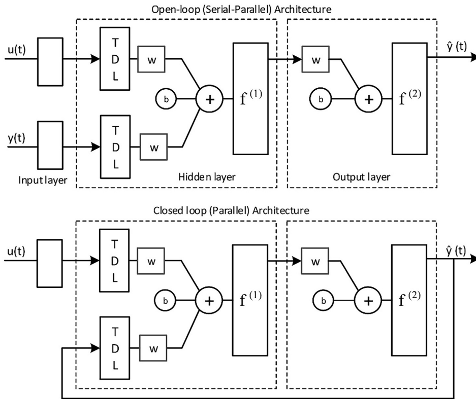
Fig. 4. The architecture of the NARX model applied in this work: TDL denotes tapped delay lines, w is a respective input or output weight, b is the bias term and f^{(1)} and f^{(2)} are activation functions in the hidden and output layer, respectively.
