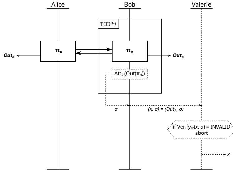
Fig. 1. Our modified protocol Clone_B(\pi) , with a TEE added and additions to the protocol shown in dashed lines. In this three-party protocol, we take the original protocol \pi = (\pi_A, \pi_B) —which does not use the TEE shown—and convert Bob's part into a program \mathcal{P} that executes his component \pi_B before producing an attestation to its output. No change is made to Alice's part of the protocol—the modifications are completely invisible to her. Valerie can then verify the attestation, and knowing that the program \mathcal{P} attests to the output of \pi_B , concludes that the protocol was correctly executed. The protocol is so-named because, in general, it takes a functionality and 'clones' one of its outputs, so that Valerie will always output the same value as the one being cloned.
