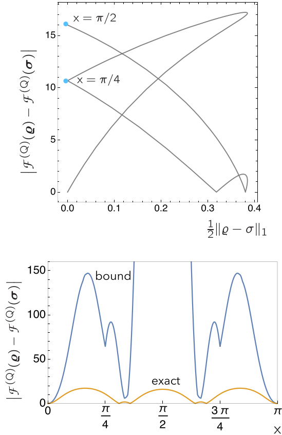
FIG. 3. (Top) Difference of the QFIs for two density matrices given in Sec. IV A vs their distance, for x \in [0, \pi/2] . It is evident, from the multivaluedness of |\mathcal{F}^{(Q)}(\varrho) - \mathcal{F}^{(Q)}(\sigma)| at the point where \|\varrho - \sigma\|_1 = 0 , that at x = \pi/4, \pi/2 the QFI exhibits violation of the reduced continuity (while satisfying the continuity in the general sense of Theorem 1). (Bottom) Comparison of the exact value of |\mathcal{F}^{(Q)}(\varrho) - \mathcal{F}^{(Q)}(\sigma)| and our upper bound (28).
