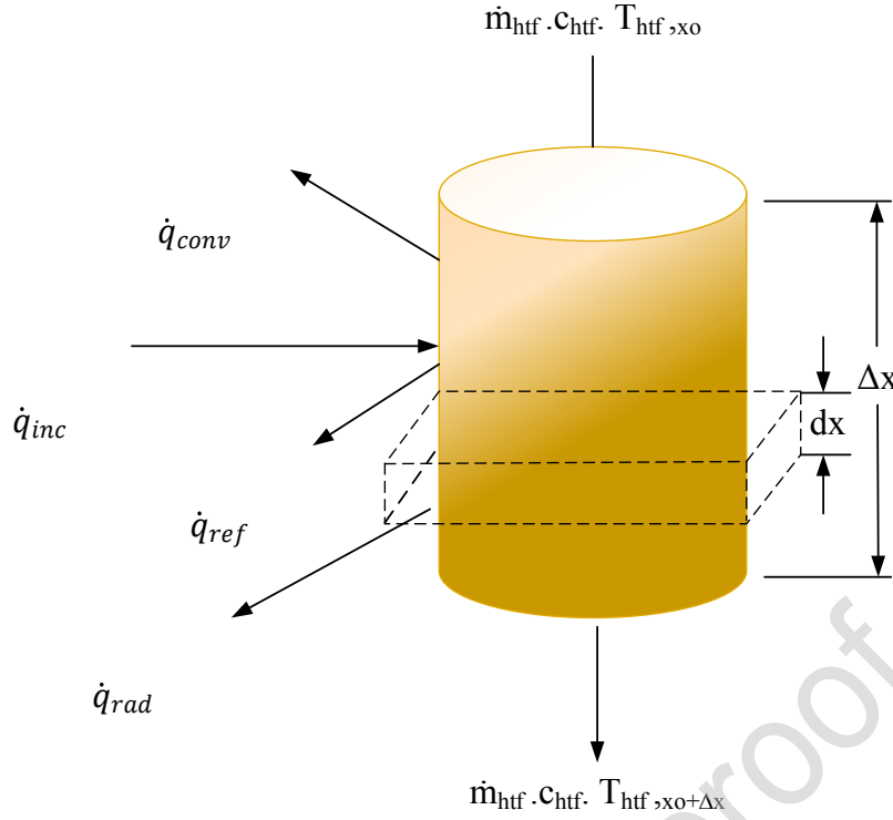
Fig. 3. Energy balance for a receiver tube element.
