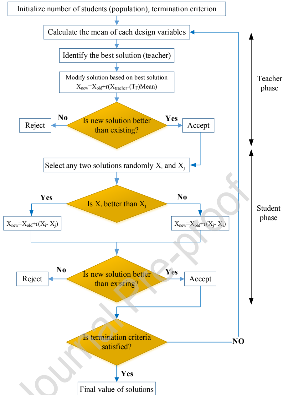
Fig. 5. A schematic of TLBO algorithm [56].
