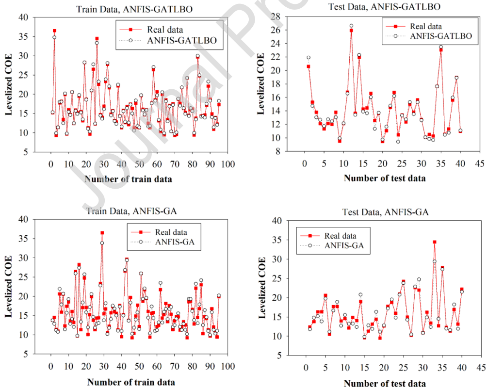
Fig. 13. Train and test data for ANFIS-GATLBO and ANFIS-GA for estimating the levelized COE.
