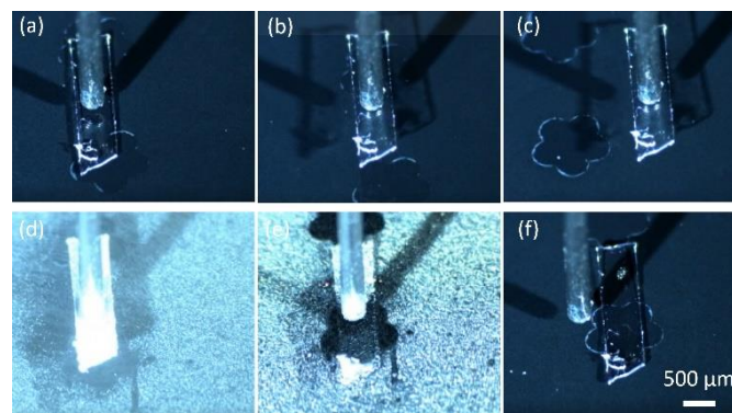
Figure 6. Capillary transport of miniature elastic ribbon. (a) a needle is above a ribbon; (b) the ribbon is picked up by the needle; (c) the ribbon is transported to the target location; (d) water mist is introduced; (e) the ribbon is released on the target site; (f) water droplets evaporate. The images are snapshots from the Supplementary Video S1.
