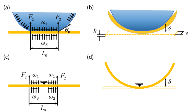
Figure 7. Electro-capillary transport scheme: (a,b) force illustration; (c,d) deformation model of a ribbon as the deflection of a cantilever beam.
