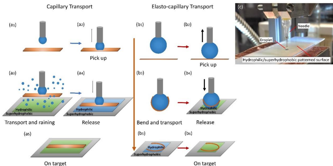
Figure 1. Schematic and system setup for transport of miniature elastic ribbons using capillary transport and elasto-capillary transport scheme. (a 1 ) and (b 1 ) A droplet is produced with a needle; (a 2 ) and (b 2 ) the needle with the droplet picks up the ribbon; (a 3 ) the ribbon is transported to the hydrophilic/superhydrophobic patterned surface and water mist is introduced; (b 3 ,b 4 ) the ribbon bends and is transported to a hydrophilic/superhydrophobic patterned surface; (a 4 ) and (b 5 ) the water film is formed on the hydrophilic site and the ribbon is released on the hydrophilic site; (a 5 ) and (b 6 ) the ribbon is on target; (c) system setup for transport of elastic ribbon.
