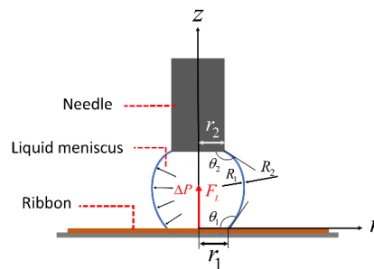
Figure 2. Force illustration of lifting a ribbon.
