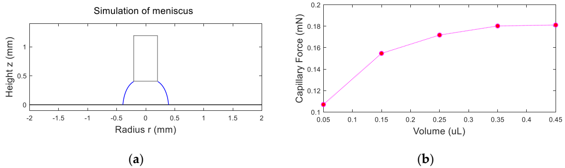
Figure 3. Simulation of meniscus and capillary lifting force analysis: (a) simulation of water meniscus of 0.15 \mu L with double iteration method; (b) capillary lifting force as the function of volume of the meniscus.
