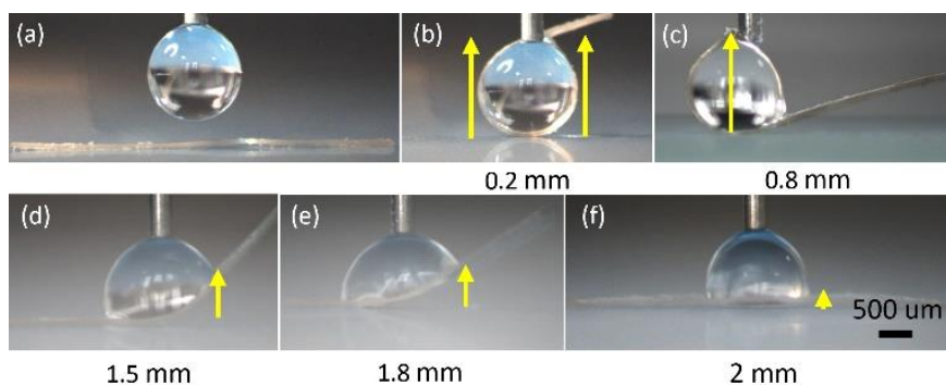
Figure 10. Deformation of the ribbon with different width. (a) A 1 \mu L droplet is dispensed at the middle of the ribbon; the ribbon with width of (b) 0.2 mm, (c) 0.8 mm, (d) 1.5 mm, (e) 1.8 mm, and (f) 2 mm bend. The deformation of the ribbon is highlighted with yellow arrow line.
