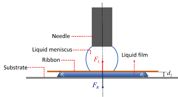
Figure 4. Force illustration of releasing a ribbon.
