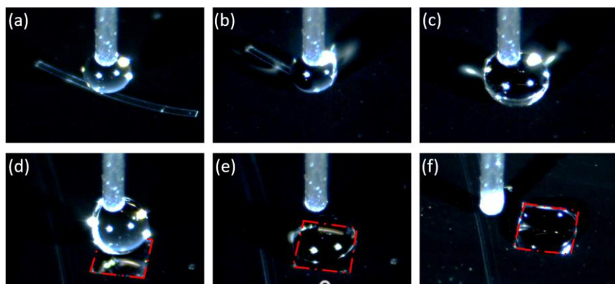
Figure 9. Elasto-capillary transport of miniature elastic ribbon. (a) a droplet is produced with a needle; (b) the needle with the droplet picks up the ribbon; (c,d) the ribbon bends and is transported to the hydrophilic site; (e,f) the droplet is in contact with the hydrophilic site and the ribbon is released on the target. The images are snapshots from the Supplementary Video S1.
