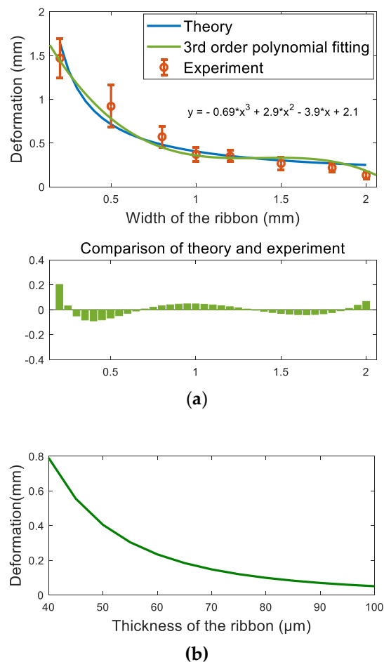
Figure 8. Influence of the width and thickness on the deformation of the ribbon. (a) deformation as the function of the width and comparison of the theoretical estimation and experiments; (b) deformation as the function of the thickness.
