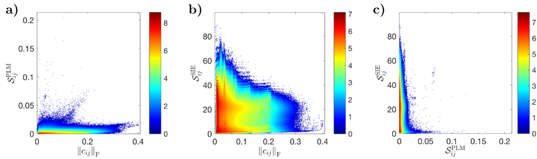
Figure 3. Pair-wise density plot of coupling strength quantified by correlations, PLM scores and SIE scores: (a) PLM scores versus correlations; (b) SIE scores versus correlations; (c) SIE scores versus PLM scores. The area inside axes is divided into 300 \times 300 cells and the colour indicates \log_{10}(\text{count}) inside each cell. Same data and same norms as in figures 1 and 2. The numerical scale in each direction depends on the details of the norms and inference procedure, e.g. PLM scores depend on \ell_2 regularization parameters. Correlations and PLM scores are numerically similar while SIE scores are not, as discussed in text.
