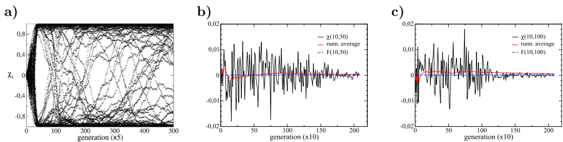
Figure 4. Temporal behavior of (a) all magnetizations defined as \chi_i = f_i(2) - f_i(1) and ((b) and (c)) two selected correlations defined as \chi_{ij} = f_{ij}(1, 1) - f_{ij}(1, 2) - f_{ij}(2, 1) + f_{ij}(2, 2) in a simulation of a population of Ising genomes (two alleles per locus). Number of loci L of the genotypes is 256, number of genotypes N in the population is 50 000, other simulation parameters as reported in table F1. Data is taken every five generations, total simulation time is 2500 generations.
