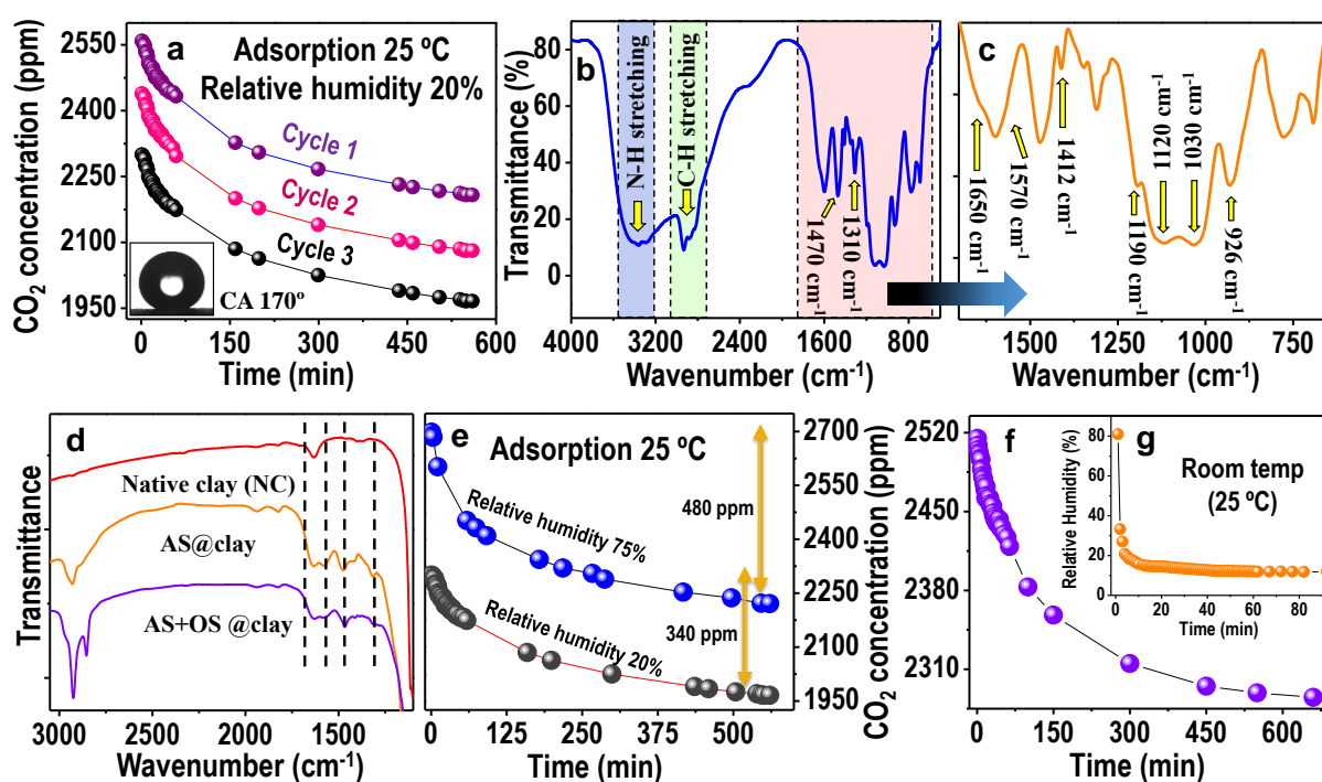
Figure 5. a, CO 2 capturing phenomenon over superhydrophobic surface at constant temperature.
