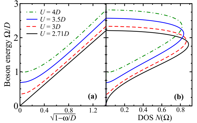
FIG. 1. The doublon/holon energy spectrum (a) and the corresponding spectral density of states (b) for different U .
