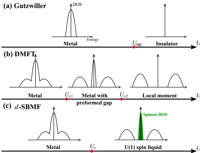
FIG. 6. Schematic diagram of the Mott transition. (a) Gutzwiller with U_{BR} \simeq 3.40D ; (b) DMFT with U_{c1} \simeq 2.38D and U_{c2} \simeq 3.04D [38,40,41]; and (c) present dynamical SBMF theory with U_c \simeq 0.8U_{BR} \simeq 2.71D . D : Half bandwidth.
