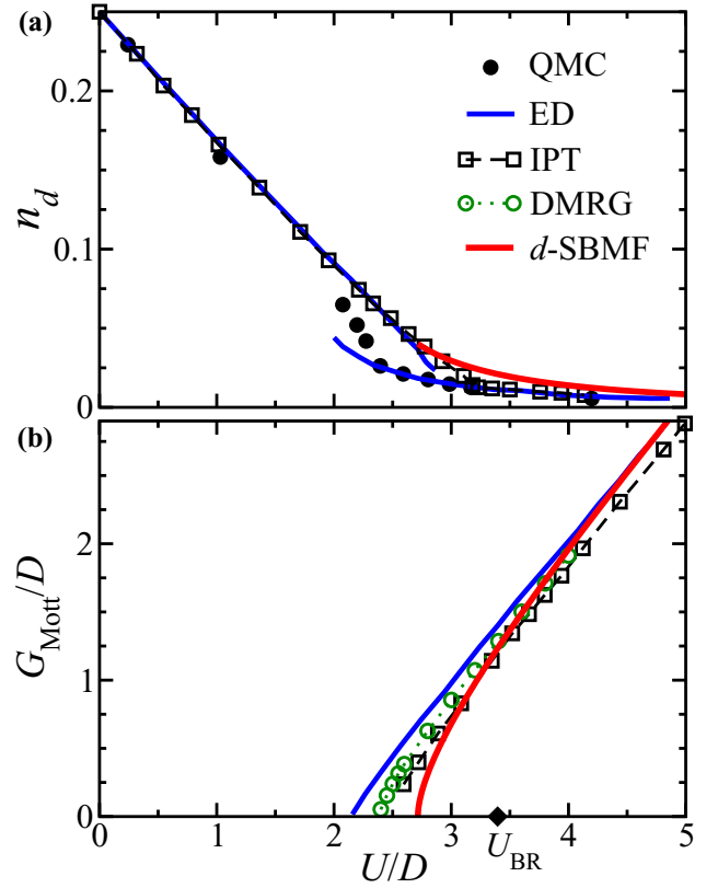
FIG. 2. Mott insulator in the large- z limit of the dynamical SBMF theory ( d -SBMF). (a) The doubloon density as a function of U . (b) The Mott gap in the charge sector as a function of U . The DMFT results obtained using different impurity solvers are also shown for comparison (data from Refs. [38,40]: Quantum monte carlo (QMC), exact diagonalization (ED), iterative perturbation theory (IPT), and dynamical density matrix renormalization group (DMRG)).
