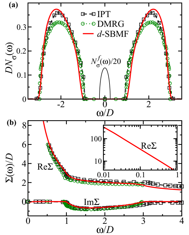
FIG. 4. Spectroscopy of the Mott insulator in the large- z limit of the dynamical SBMF theory (red lines) at U = 4D . (a) The spectral density of states. Thin solid line: Spinon density of states. (b) The real and imaginary parts of the electron self-energy. Inset: Real part of self energy on log-log plot, showing the 1/\omega dependence. The DMFT results obtained at U = 4D using the zero temperature IPT (open squares) [38] and the dynamical DMRG (open circles) [40] impurity solvers are also shown for comparison.
