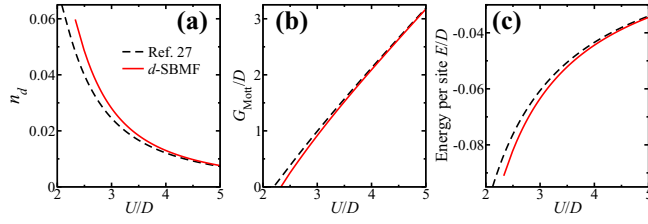
FIG. 5. Mott transition on two-dimensional square lattice obtained in Ref. [27] and the present dynamical SBMF theory. (a) Doublon density, (b) charge gap, and (c) state energy per site as a function of Hubbard U .
