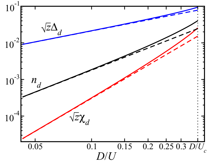
FIG. 3. Evolution of the doubloon density n_d , D/H hopping \sqrt{z}\chi_d , and D-H binding \sqrt{z}\Delta_d as a function of D/U on a log-log plot in the Mott insulating state. Solid lines: Fully self-consistent solutions of Eqs. (19)–(21). Dashed lines: Asymptotic solutions in the large- U limit given in Eqs. (29)–(31). The vertical dotted line indicates the critical D/U_c \simeq 0.37 .
