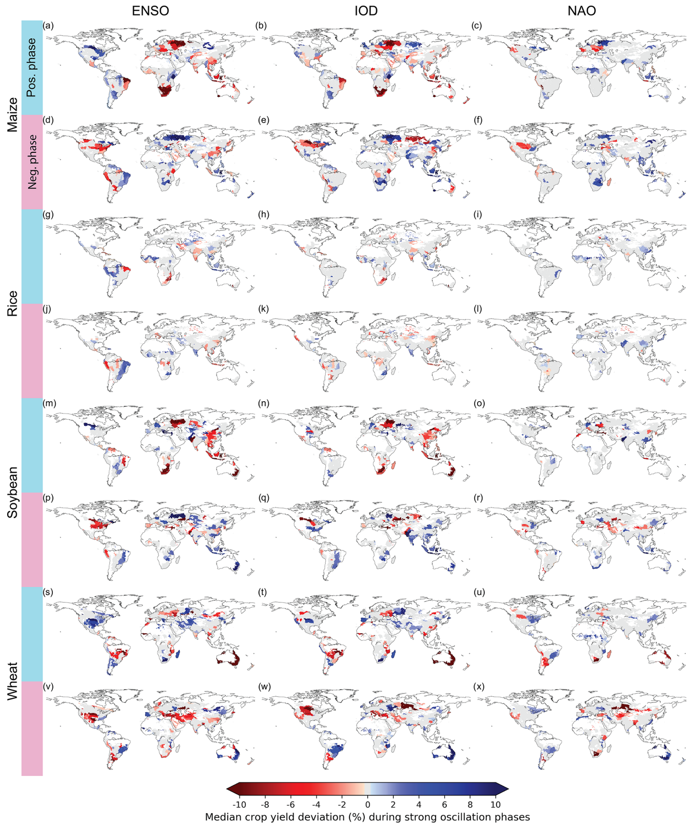
Figure 2. Actual maize (a–f), rice (g–l), soybean (m–r), and wheat (s–x) yield anomalies during strong phases of ENSO, IOD, and NAO at the FPU scale. The anomaly values are derived from a sample including crop yield data from all GCMs that simulate the crop in question with the AgMERRA climate input. Statistically insignificant ( p > 0.1 ) anomaly values are marked as zero (grey). White denotes that the crop in question is not produced in that area. Patterns are discussed in Sect. 3.1 and 3.2.
