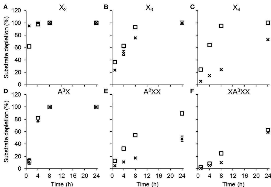
FIGURE 2 | Substrate depletion by AbPDH1 (square) and AmPDH1 (cross) followed by HPAEC-PAD. Substrates: (A) xylobiose, X_2 , (B) xylotriose, X_3 , (C) xylotetraose, X_4 , (D) 3 2 - \alpha -L-arabinofuranosyl-xylobiose A^3X , (E) 2 3 - \alpha -L-arabinofuranosyl-xylotriose, A^2XX , and (F) 3 3 - \alpha -L-arabinofuranosyl-xylotetraose XA^3XX . Depletion of 5 mM substrate using 0.2 U/ml PDHs, 1 mM BQ and 0.2 U/ml laccase was compared to the control reaction containing all reaction components except PDH. Error bars show the data range of duplicate reactions. Error bars are not visible when the data range fits inside the drawn data point.
